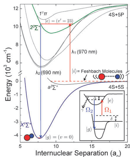
Fig. 8 Schematic of the transfer from KRb Feshbach molecules to the absolute rovibrational electronic ground state. The intermediate state was chosen to be the v' = 23 state of the nominally 2^3\Sigma^+ electronically excited potential for its good wavefunction overlap to both the Feshbach molecules and the absolute ground-state molecules. The three levels are coupled by two lasers that have the laser wavelength of \lambda_1 (970 nm) and \lambda_2 (690 nm) and are both referenced to a stable optical frequency comb. (Inset) Diagram showing the parameters that describe a coupled three-level system, where \Omega_1 and \Omega_2 describe Rabi frequencies for the two transitions.
