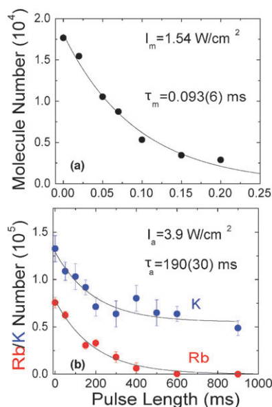
Fig. 6 Comparison of the optical excitation rate from Feshbach molecules to the v' = 23 state of the excited 2^3\Sigma^+ potential and (b) from a near quantum degenerate gas of atoms to the same excited state. The measured depletion of the molecule/atom population is due to excited \text{KRb}^* formation followed by spontaneous decay and loss from the system. The \text{KRb}^* formation rates were characterized by the exponential time scales, \tau_m and \tau_a , respectively. The enhancement factor for starting from Feshbach molecules instead of atoms near the Fano–Feshbach resonance is \frac{\tau_a/I_a}{\tau_m/I_m} \approx 5000 .
