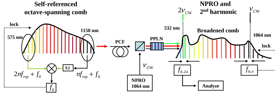
Fig. 1. After passing through an f - 2f interferometer for self-referencing, the remaining spectrum (600–1100 nm) from the octave-spanning frequency comb is broadened in photonic crystal fiber (PCF) and overlapped with the output of an NPRO Nd:YAG at 1064 nm. The resulting heterodyne beat, f_{b,n} , and the carrier envelope offset frequency, f_0 , are locked to RF references. Polarization-selective doubling of the overlapped beams ensures that only the CW light is frequency doubled, while collinear beam propagation reduces technical noise. The out-of-loop beat at 532 nm, f_{b,2n} , is analyzed as detailed in the text.
