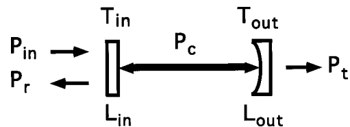
Fig. 1. Conversion of incident power into reflected, built-up, and transmitted powers. T_{in} , T_{out} and L_{in} , L_{out} , transmissions and losses of input and output coupling mirrors, respectively. P_{in} , P_r , P_t , cavity input and reflected and transmitted light powers, respectively. P_c , one-way circulating light power.
