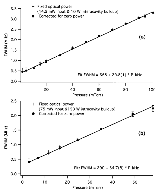
Fig. 12. Pressure-broadening measurement of the overtone transitions. (a) P(11) line in the (\nu_1 + 3\nu_3) overtone band of C_2H_2 at 790 nm. (b) P(5) line in the (\nu_2 + 3\nu_3) band of C_2HD at 1064 nm.
