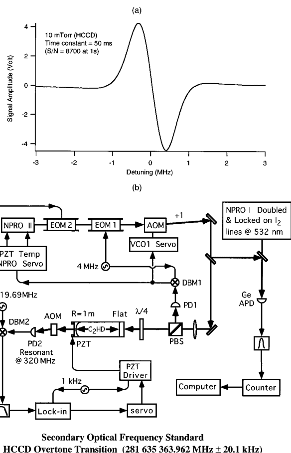
Fig. 15. (a) NICE OHMS signal used for locking the NPRO-cavity system onto the C_2HD resonance. (b) Experimental setup for heterodyne beat between the two MISER systems, one locked on the C_2HD resonance and the other frequency doubled and locked onto an I_2 reference at 532 nm. Abbreviations defined in text and previous figure captions.
