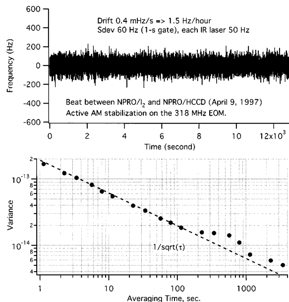
Fig. 16. Time record of the beat frequency between the two NPRO's. The frequency offset of 5252.2254 \pm 0.0026 MHz in the beat is suppressed. The Allan variance is calculated from these data.
