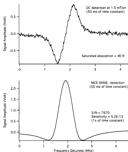
Fig. 11. Estimation of noise-equivalent sensitivity based on the S/N obtained by the NICE-OHMS technique and the saturated absorption level measured by dc detection.
