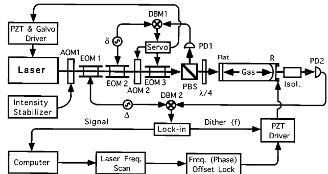
Fig. 5. Experimental configuration for NICE-OHMS. An external stabilizer (AOM–EOM) is employed to widen the frequency servo bandwidth. Sidebands at \delta/2\pi = 4 MHz are used for reflection lock to cavity; sidebands at \Delta = \text{cavity FSR} are used in transmitted light as local oscillators for heterodyne detection of saturated gas absorption inside the cavity. DBM's, double-balanced mixers; PD's, photodiodes; R, concave reflector; other abbreviations defined in text.
