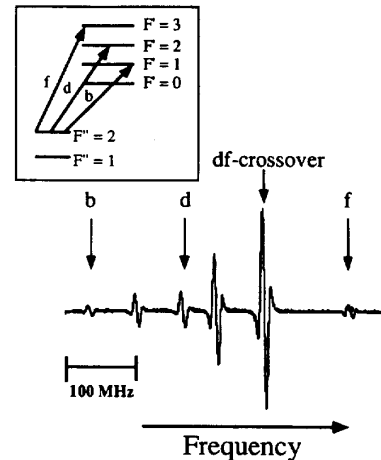
Fig. 2. Frequency scan over the hyperfine components in 87 Rb. Assignment of the components is indicated.
