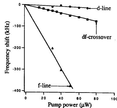
Fig. 3. Optical frequency shifts induced by laser power. The probe power used was 10 μW. One notices the strong shifts of the f -component, which arises from the closed 2-level transition F'' = 2 \rightarrow F' = 3 , whereas the d -component ( F'' = 2 \rightarrow F' = 2 ) corresponds to an open transition and has a much smaller shift. See text for details.
