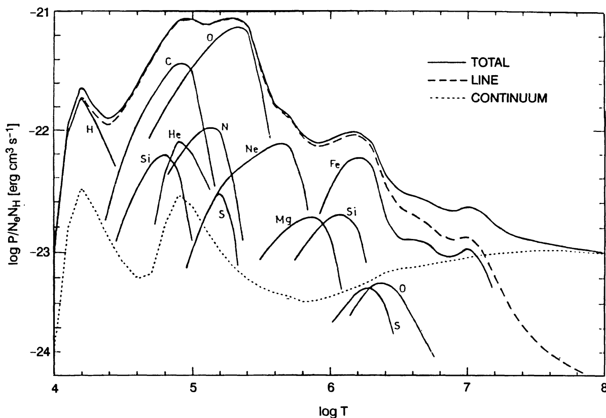
Figure 6 The total emissivity and contributions from individual elements in the 1–2000-Å spectral region (from Landini & Monsignori-Fossi 1990).
