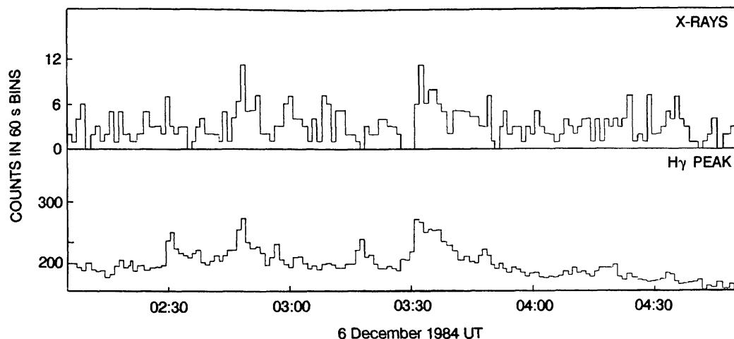
Figure 8 The SXR flux of UV Ceti as measured by Exosat versus H\gamma peak as seen by the ESO 3.6-m telescope (from Butler et al 1986).
