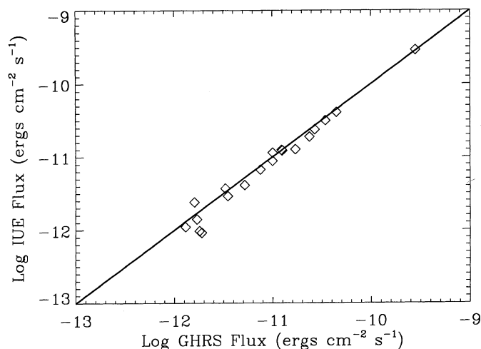
FIG. 2.—Comparison of emission line fluxes measured from the GHRS G140L spectra and the composite low-dispersion IUE spectrum of Capella. The solid line corresponds to equal GHRS and IUE line fluxes.
