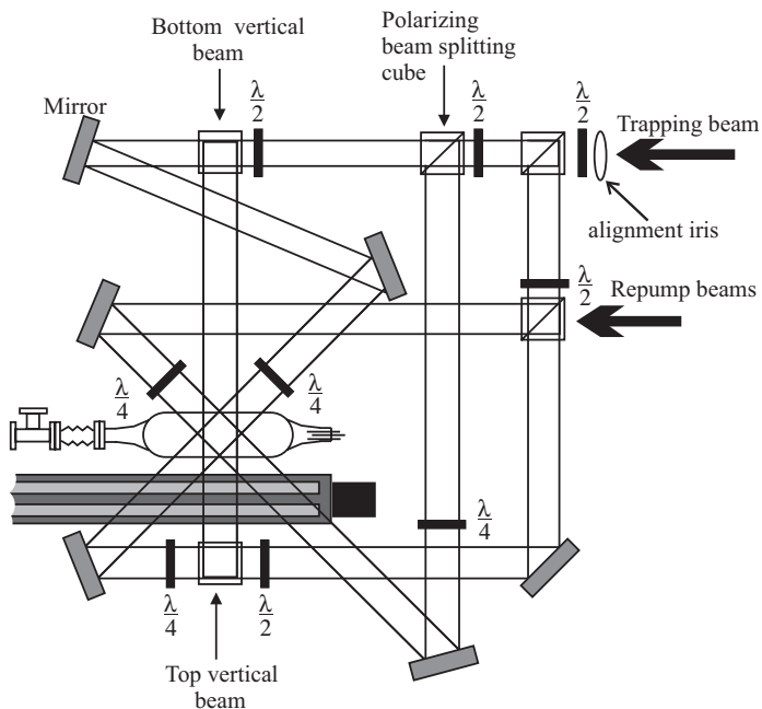
Fig. 7. Schematic of the MOT optical layout (top view). The linear track and servo motor are shown in their approximate locations on the table. Some of the mirrors and waveplates for the vertical beams are not shown. There are enough degrees of freedom to adjust the position and angle of each beam.
