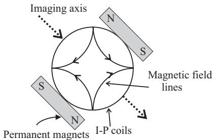
Fig. 14. Ioffe–Pritchard magnetic trap (end on view). The permanent magnets are at a 45^\circ angle with respect to the horizontal axis so as to provide a magnetic field in the same direction as the magnetic field from the quadrupole trap used to transport the atoms. The magnetic trap can be rotated by 45^\circ and still confine the atoms as they are brought into the IP trap region by the quadrupole coils. Four permanent magnets, magnetized through the thin dimension, will also work to provide a two-dimensional quadrupole field with no field along the axial direction of the trap. However, using just two magnets magnetized through the thin direction would create a significant gradient along the axial direction of the trap, which would interfere with the transport of atoms via the moving quadrupole trap.
