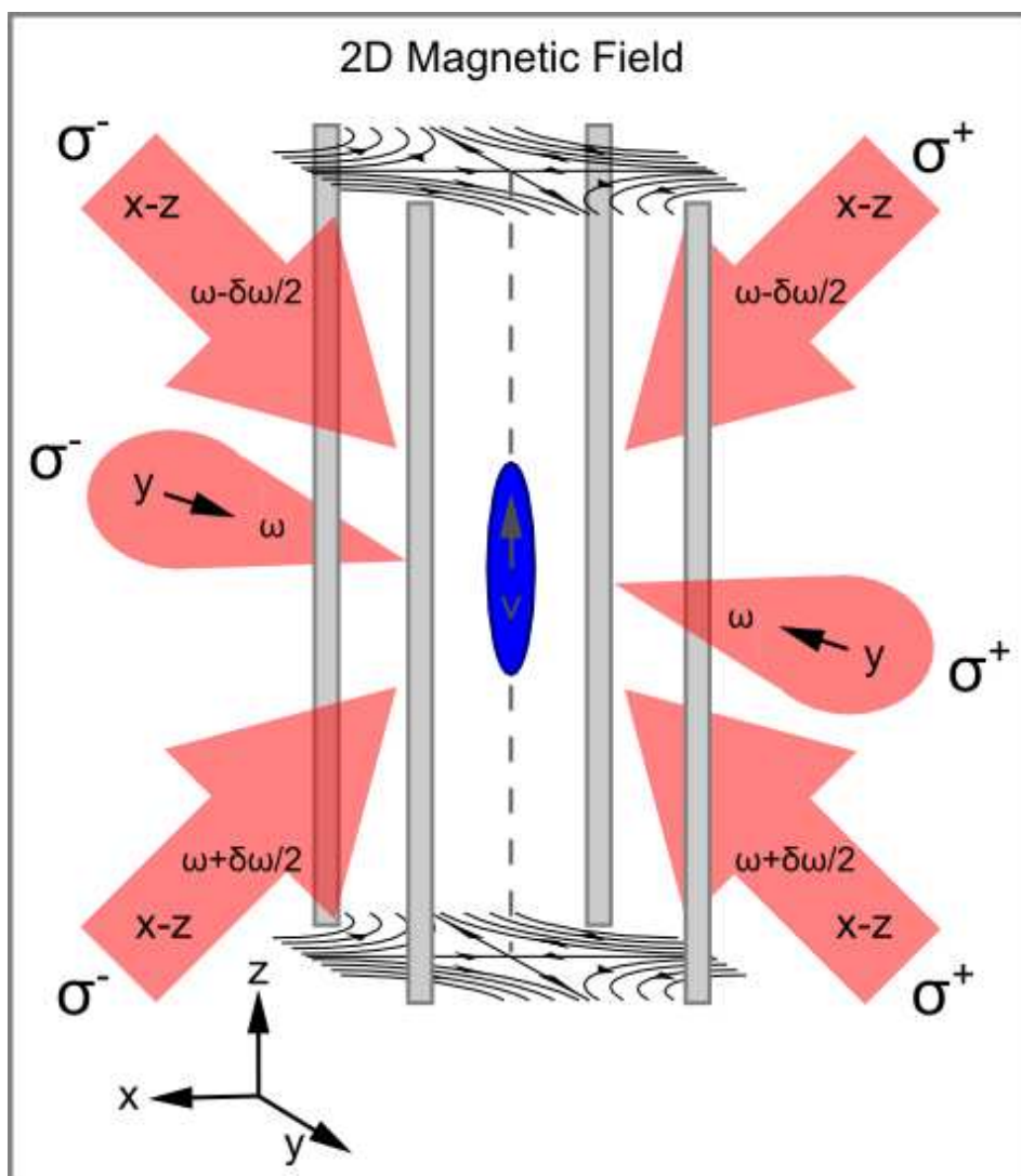
Figure 2.6: (Color) Moving molasses magneto-optical trap diagram. Four independent counter-propagating beams enter the cell at an angle of 45^\circ in the x - z plane and are shifted by \pm\delta\omega from the center frequency \omega to create a net velocity for the atoms upward. A retro-reflected beam enters the cell along the y -axis direction to provide a confining force along the third dimension of the trap.
