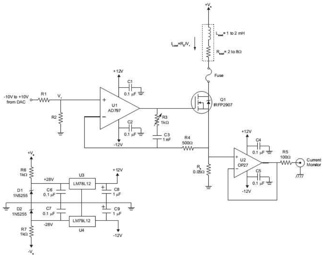
Figure A.1: Unipolar coil driver circuit diagram.
