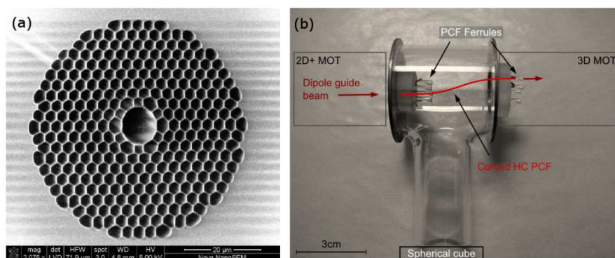
Figure 6.4: (Color) (a) Cleaved facet of the NKT HC-1060-02 hollow core photonic crystal fiber for 1060 nm. At the center is the 10\ \mu\text{m} hollow core where a red detuned 1064 nm dipole beam would guide atoms with a mode field diameter of 7.5\ \mu\text{m} . (b) Photo of the partially assembled PCF atom transport test cell. The 2\text{D}^+ MOT cell is on the left, where the atom source is located. The dipole guide beam is coupled through the 2\text{D}^+ MOT cell, and guides atoms through the connecting T-shaped chamber where they can be captured in a 3D MOT, a dipole trap, or detected, on the right.
