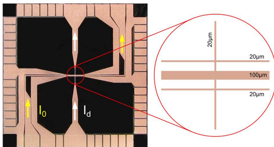
Figure 3.7: (Color) A photo of the atom chip designed for direct evaporation. There are three main traces, one with a 100\ \mu\text{m} width and two that run parallel to it with a 20\ \mu\text{m} width. There is one dimple trace that runs down the middle of the chip, which tapers to a 20\ \mu\text{m} width at the center of the chip where it crosses the main wires.
