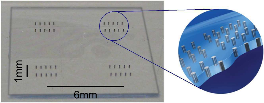
Figure 6.2: (Color) SCHOTT HermeS glass for source tube electrical feedthroughs. Left is a 12 mm \times 12 mm square of the HermeS glass cut on a wafer dicing saw. Right is a diagram of the coplanar tungsten pins.
