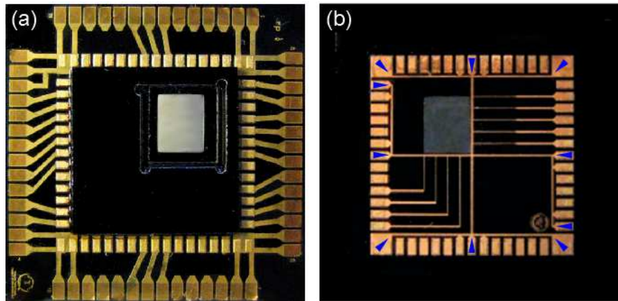
Figure 3.6: (Color) A photo of the atom chip used in the V2 channel cell.(a) The ambient side of the atom chip. A window is etched into the chip inside the electrical connection pads and feedthrough via metallization. A Pyrex window is anodically bonded to this side to seal vacuum. (b) The main wires, indicated with arrows at the vias, form a cross in the center of the chip. They were designed to use redundant vias and allow for a dimple trap in either orientation. The thinner wires can be used to form a T-trap in several locations.
