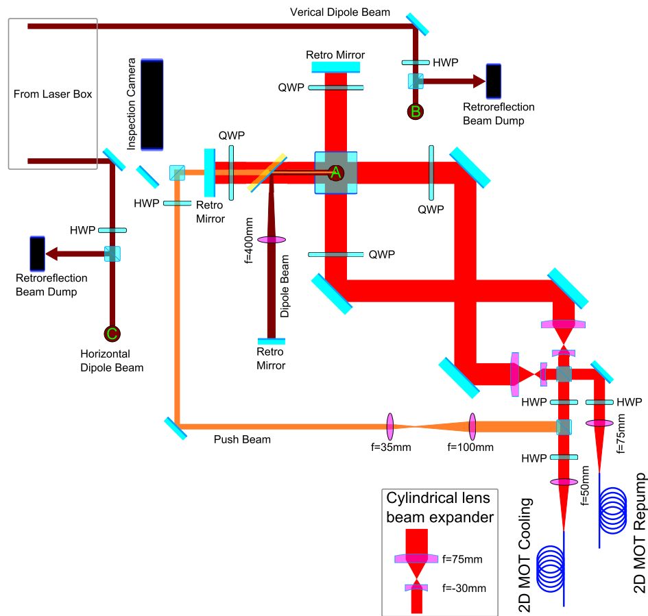
Figure 5.13: (Color) Tier 1 diagram of the vertical chamber setup, the 2D^+ MOT. The cooling fiber was collimated by an f=50 mm achromat, with some light picked off for the push beam. The light was split and sent through a 2.5:1 cylindrical beam expander. A quarter waveplate made the light circularly polarized when it was sent into the cell and retroreflected. The push beam was shrunk in a 3:1 telescope and sent into the cell vertically. The dipole beams came from the laser box via free space on the left, where they were directed to tier 3 of the optical setup. The vertical dipole beam was sent upward at point B. The vertical dipole beam was sent downward from tier 3 through the cell, where it exited the cell at point A. The horizontal dipole beam was sent upward at point C.
