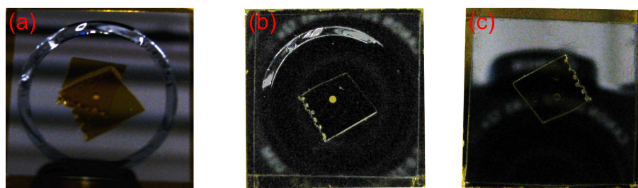
Figure 3.4: (Color) Sequence of silicon pinhole recovery via HF removal of glass. The pinhole, 2D^+ MOT chamber optical faces, and 2D^+ MOT chamber anodic bond with the silicon have been protectively masked with Kapton tape. (a) Silicon after anodic bonding with a clearly visible ring of Pyrex and no HF etching. (b) Silicon with some HF etching showing the removal of the lower portion of the ring. (c) Silicon after successful HF etching.
