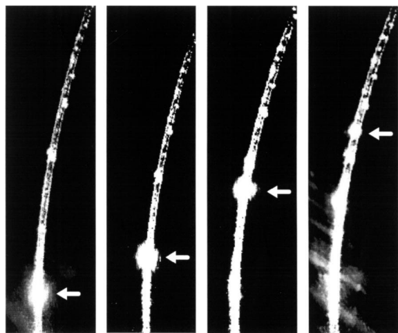
FIG. 1. Snapshots in time showing the levitation of a water droplet in a 30- \mu\text{m} , air-filled hollow fiber. In each snapshot, a 5-mm section of 20-mm long fiber is imaged on a CCD camera. The bright scattering of light by the droplet, indicated by the arrow, is easily seen by the naked eye as the water droplet travels upward through the curved region. Bending the fiber is accomplished by translating the output tip while holding the input end fixed.
