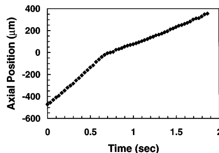
FIG. 3. Measurements of axial position with time of a 7- \mu\text{m} diameter polystyrene sphere optically guided from bulk fluid into a 20- \mu\text{m} diameter fiber. The position z = 0 corresponds to the fiber input tip. The particle velocity (slope of curve) abruptly decreases when the sphere enters the fiber as a result of increased drag.
