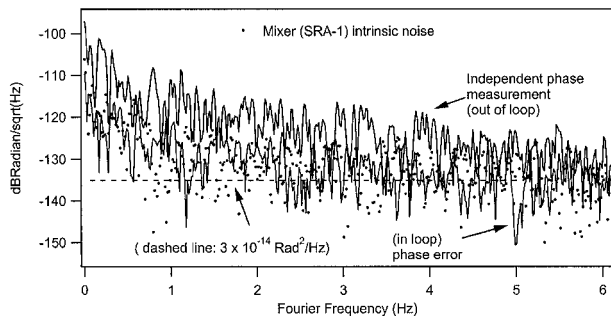
Fig. 3. Frequency spectrum of the mixers' output, indicating the phase-noise spectral density inside (lower solid curve) and outside (upper solid curve) the servo loop. The dotted curve is calibration of the noise floor for the mixer.
