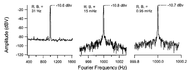
Fig. 2. Fourier spectra of the optical heterodyne beat signal after it was downconverted to a 1-kHz carrier frequency. R.B.'s, resolution bandwidths of the analyzer.
