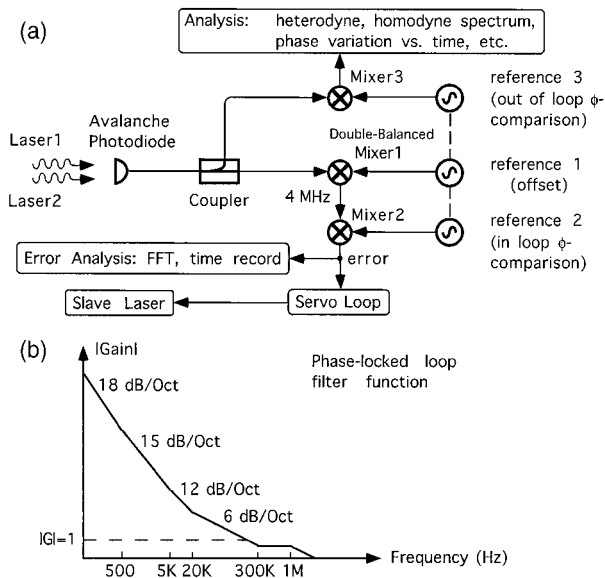
Fig. 1. (a) Experimental setup for the optical PLL between two Nd:YAG lasers. All rf reference oscillators share a common time base. (b) Filter transfer function of the PPL. Break points of the gain curve are indicated by frequency marks on the horizontal axis. A 6-dB/octave roll-off corresponds to a first-order integrator.
