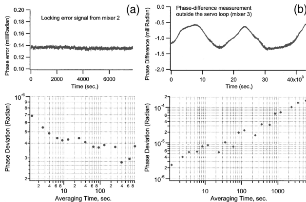
Fig. 4. Time records of the phase measurement inside (a) and (b) outside the servo loop. Phase Allan variances are calculated from these time records.
