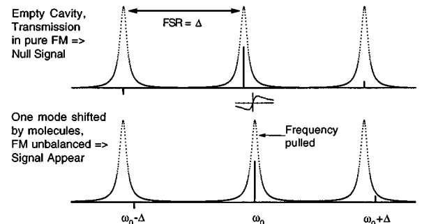
Fig. 1. Optical spectrum and the detection principle for NICE-OHMS.
