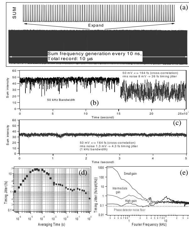
FIG. 5: Timing jitter noise analysis. (a) A 10\ \mu\text{s} direct digitization record of the sum frequency generation. Also shown is the time-expanded trace. The pulse-to-pulse intensity fluctuation is below 0.4%, similar to the original laser intensity fluctuation. (b) Sum frequency generation observed with a 50 kHz bandwidth. The left trace shows two pulses optimally overlapped and the right trace shows two pulses offset by a half width. (c) Sum signal observed under a 160 Hz bandwidth, showing an rms timing jitter noise of 4.3 fs. (d) Allan variation of the timing stability, showing the maximum jitter occurs around 10 - 100 \mu\text{s} . (e) Fourier frequency spectrum of the error signal from the 8 GHz phase locked loop.
