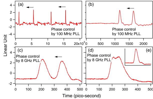
FIG. 3: Control of the relative timing offset between the two independent pulse trains using the combined phase locked loops. Relative to laser #1, the pulse train from laser #2 is scanned via the rf phase shifter in the PLL. (a) Two independent pulse trains incident on a same photodiode, with repetition period of 10 ns. (b) Expanded time axis, 100 MHz PLL control. (c) Time scale further expanded, 8 GHz PLL control. (d) Two pulses nearly overlapped via adjustment of the 8 GHz phase shifter. (e) Two pulses maximally overlapped, permitting study of relative timing jitter.
