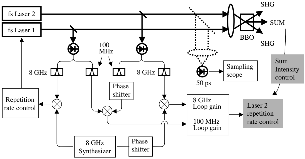
FIG. 1: Experimental setup for timing synchronization of two fs lasers. The three phase locked loops for synchronization are shown, along with the signal analysis scheme.
