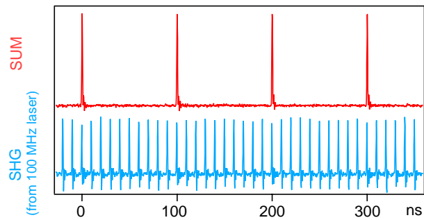
FIG. 6: Sum frequency generation from two synchronized fs-lasers that have different repetition rates, one at 90 MHz and the other at 100 MHz. The second harmonic signal from the 100 MHz laser is also shown. Notice the slight decrease in the second harmonic signal when sum frequency generation occurs with two pulses overlapped.
