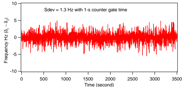
FIG. 7: Record of the carrier beat signal between the two fs lasers when they are synchronized and phase locked. The beat frequency under the locked condition shows a standard deviation of 1.3 Hz at 1-s averaging time.
