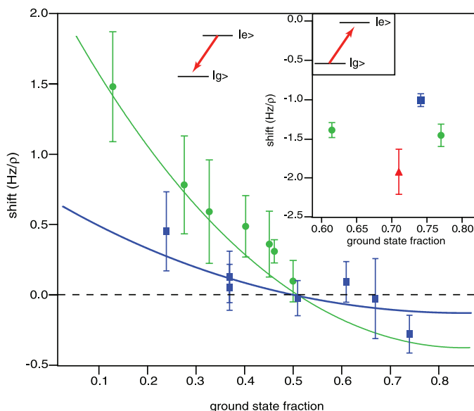
Fig. 2. Measured density-dependent frequency shift as a function of the final excitation fraction and temperature. Atoms are initially spin polarized and transferred to {}^3P_0 ( |e\rangle ) before the spectroscopy pulse is applied. The squares (circles) show the measured shift for T = 1 (3) \mu\text{K} . The lines show the calculated shifts when the two-atom model is used with only a single scaling factor. Near \sim 50\% the shift goes through zero. In the inset, the measured shift is shown for atoms excited from the {}^1S_0 ( |g\rangle ) state for T = 1 \mu\text{K} (squares), 3 \mu\text{K} (circles), and 5 \mu\text{K} (triangles). However, the magnitude in this case could be influenced by imperfect spin polarizations. For both plots, as the temperature is decreased, the inhomogeneity also decreases, leading to a smaller collision shift. \rho is the atomic density of 10^{11}/\text{cm}^3 . The density-dependent shift for each excitation fraction is determined with an interleaved scheme in which the density is varied every 100 s. Pairs of such data are then used to determine the frequency shift. Typical data sets include 20 to 30 pairs of density comparison, with the error bars indicating the standard error (SE).
