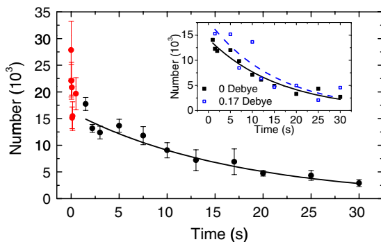
FIG. 1 (color online). Loss of ground-state KRb molecules as a function of time in a 3D lattice with depths of 56, 56, and 70 E_R in x , y , and z , respectively, where E_R = \hbar^2 k^2 / 2m is the KRb recoil energy, k is the magnitude of the lattice beam wave vector, and m the molecular mass. Neglecting the very short time points (red solid circles), the number of molecules for times larger than 1 s (black solid circles) are fit to a single exponential decay, yielding a 1/e lifetime of 16.3 \pm 1.5 s. Inset: Lifetime in an isotropic lattice with a depth of 50 E_R , with (blue open squares, 0.17 D) and without (black squares, 0 D) an applied electric field. The lifetimes at 0.17 D ( 15 \pm 4 s) and 0 D agree within uncertainty.
