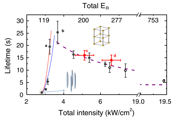
FIG. 2 (color online). Lifetime of KRb ground-state molecules in an optical lattice. Black circles: x and y lattice beams are fixed at 56 E_R per beam, while z is varied from 0 to 136 E_R (1 E_R corresponds to a lattice intensity I = 0.025 kW/cm 2 ). The lifetime reaches a maximum of 25 \pm 5 s when the z lattice depth is 34 E_R (point b). For higher lattice intensities, the lifetime decreases, which is consistent with loss due to off-resonant light scattering (dashed line). The open circles correspond to 3D lattices where the radial confinement was also varied. The red squares correspond to lifetimes measured with an additional traveling-wave beam at 1064 nm illuminating the molecules in the 3D lattice. Point c (d) corresponds to the 3D lattice of point a with an intensity of 3.2 kW/cm 2 (b with 3.7 kW/cm 2 ) plus the additional beam intensity of 2.3 kW/cm 2 (3.5 kW/cm 2 ). Solid lines: see text.
