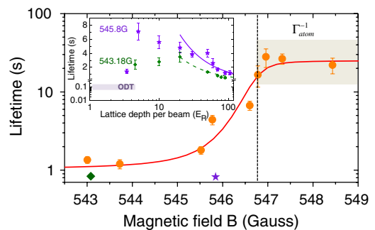
FIG. 3 (color online). Lifetime of Feshbach molecules and confinement-induced molecules measured as a function of B . A purified sample of Feshbach molecules is held in an isotropic 3D optical lattice ( 50 E_R per beam, 20 kHz trap frequency). Near the Feshbach resonance, the loss rate due to photon scattering can be modeled (solid line) as a weighted sum of the free atom loss rate \Gamma_{\text{atom}} and a higher loss rate for tightly bound molecules \Gamma_{\text{molecule}} . The grey shaded area indicates the single-atom lifetime, and its uncertainty, measured for the same experimental conditions. Inset: Lifetime of Feshbach molecules in a 3D lattice as a function of the trap intensity, at 545.8 G (blue stars) and 543.18 G (green diamonds). The dashed and solid line fits are used to extract the scattering rates.
