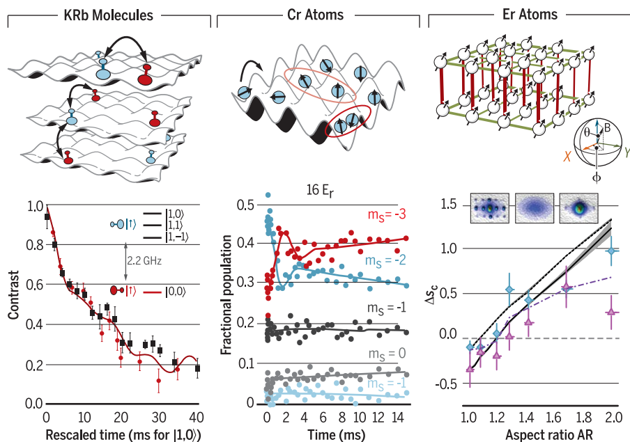
Fig. 4. Experimental observation of dipolar interactions in 3D lattices, using polar molecules and magnetic atoms. (Left) Measurement of Ramsey fringe contrast in a sparsely filled and deeply confining 3D lattice of KRB molecules with spins encoded in the two rotational states (89). (Middle) Measurement of the fractional Zeeman population in a bosonic Cr gas in a lattice. Here, |m_s| = 0, 1, 2, and 3 label the different Zeeman levels. The case shown corresponds to a lattice depth of 16E_r ( E_r is the photon recoil energy), where tunneling is largely suppressed and the spin dynamics are mainly induced by dipolar exchange processes between neighboring sites. [Adapted from (93, 94) with permission and copyrighted by the American Physical Society] (Right) Modification of the critical lattice depth of the superfluid-to-Mott insulator transition as a result of the magnetic dipolar interaction between spin-polarized Er atoms. The dipolar interaction modifies the lattice depth at which the phase transition takes place in a way that depends on the atomic cloud geometry and dipole orientation. \Delta s_c is the difference in the critical value of the lattice depth for two different dipole orientations, \theta = 0^\circ and \theta = 90^\circ . The angle was varied by changing the direction of the polarizing magnetic field. [Adapted from (95) with permission]
