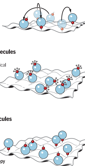
Fig. 5. A range of prospective advanced quantum materials assembled with ultracold molecules.
