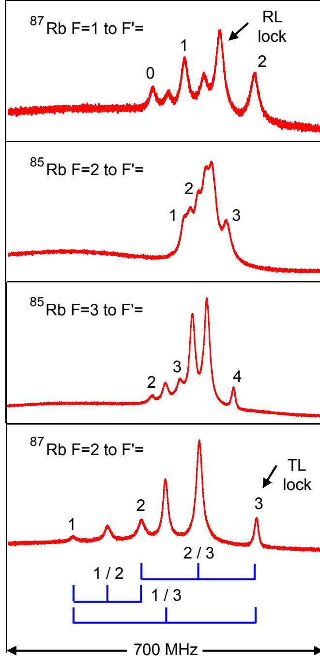
Figure 3.5: Saturated absorption spectra, showing the hyperfine structure of the 5S_{1/2} \rightarrow 5P_{3/2} transitions for the two Rb isotopes. The numbers labeling the hyperfine peaks correspond to F' states in the 5P_{3/2} manifold. Note that the spectra contain both true Doppler-free resonances (numbered peaks) and crossover resonances. The crossover resonances occur at frequencies (\nu_a + \nu_b)/2 for each pair of true resonances at frequency \nu_a and \nu_b , as exemplified for the bottom spectrum.
