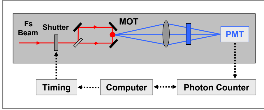
Figure 4.5: Shown here is the optical configuration for the counterpropagating beams, implemented in all our two-photon studies, including those described in Chapters 5 and 6. The 420-nm blue fluorescence detected by the PMT is sent to a photon counter and then read into the computer.
