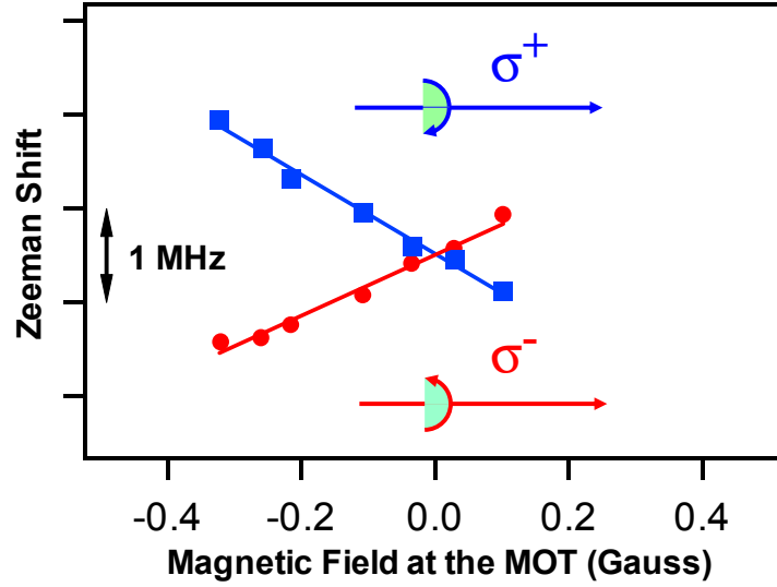
Figure 4.18: The two-photon fluorescence signal is used to cancel the residual magnetic fields: Zeeman-shifted spectra are obtained with right and left circularly polarized femtosecond comb light and the zero-frequency shift point is determined.
