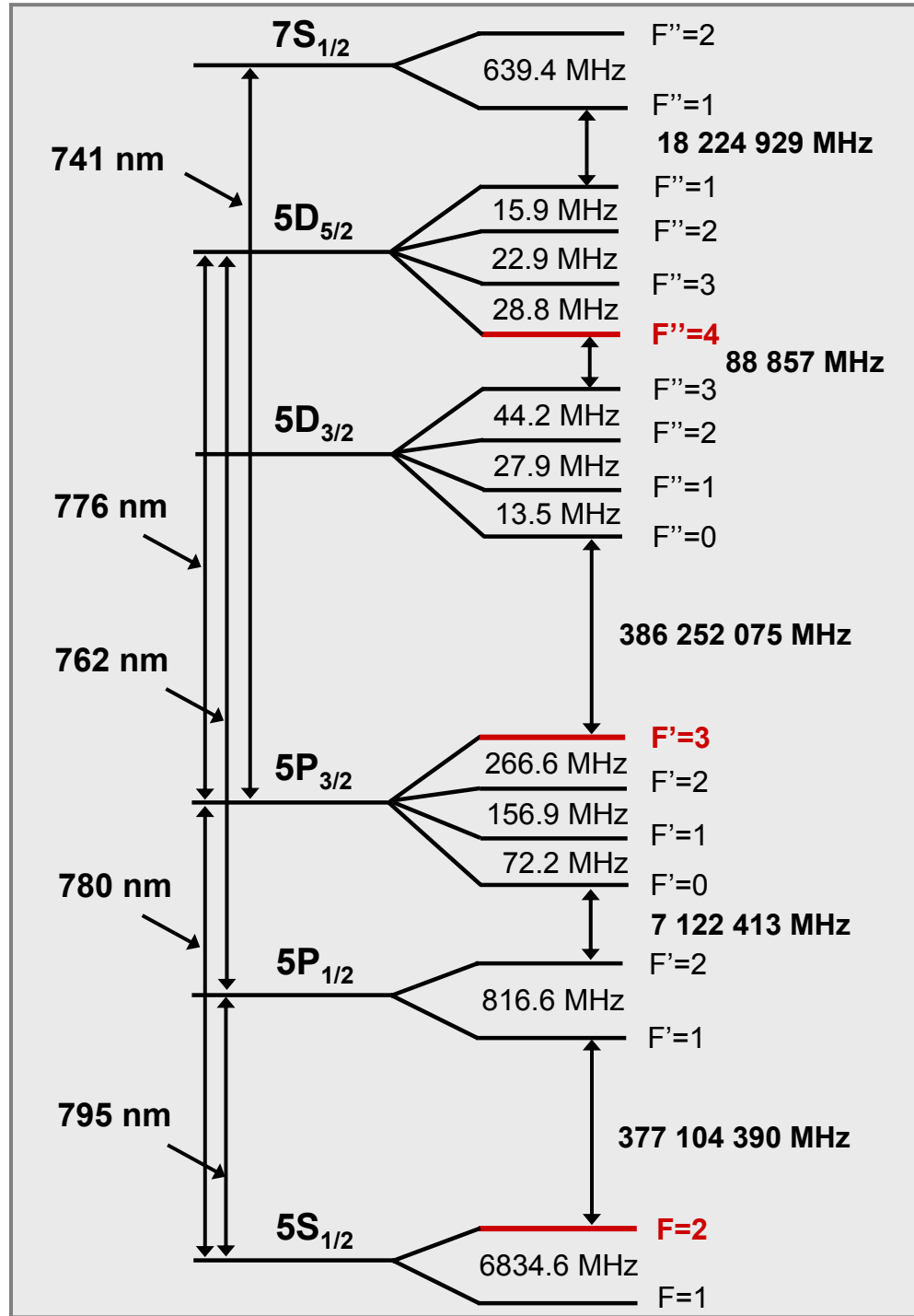
Figure 4.2: Schematic of the ^{87}\text{Rb} energy levels participating in the one- and two-photon transitions we studied, including the wavelength and energy level information. The levels highlighted in red correspond to the closed 2-3-4 transition pathway (section 4.4). We have investigated seven two-photon transitions, as detailed in section 5.2.
