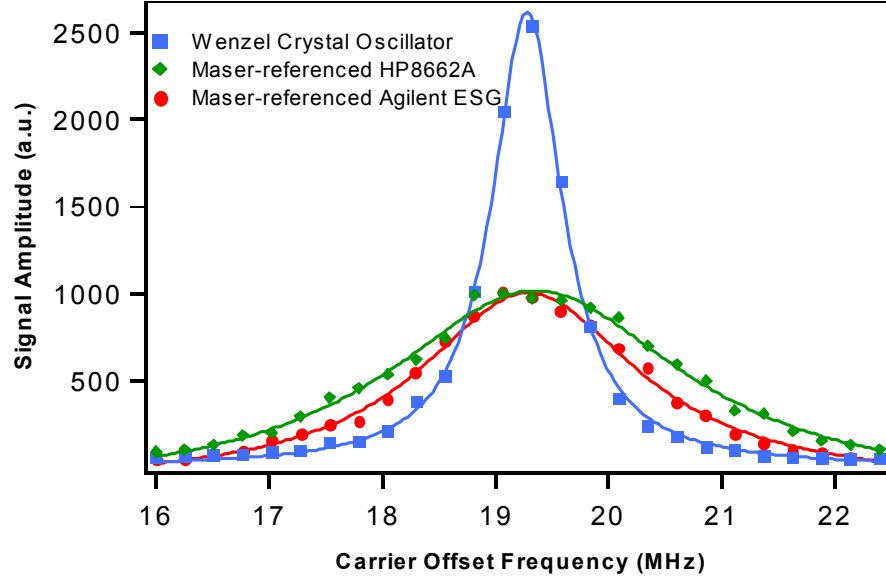
Figure 4.7: Comparison among two-photon lineshapes obtained with different rf references for the f_r lock, showing the importance of having a reference with good short-term stability.
