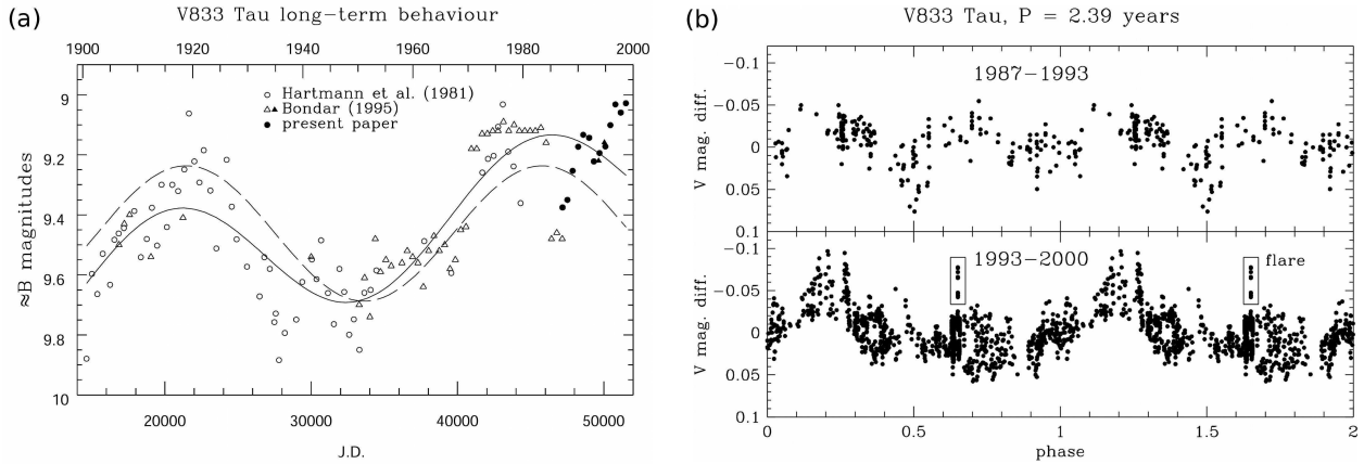
Figure 2.1: (a) Slightly more than 100 years (see upper abscissa) of photometric data from photographic and photoelectric measurements of the K7V star V833 Tau, showing a long-term Gleissberg-like modulation. (b) Short-term variability of V833 Tau, showing its shorter 2.4-year periodicity and a bright white-light flare occurring during the peak of one of these cycles (Adapted from Oláh et al. (2001)).
