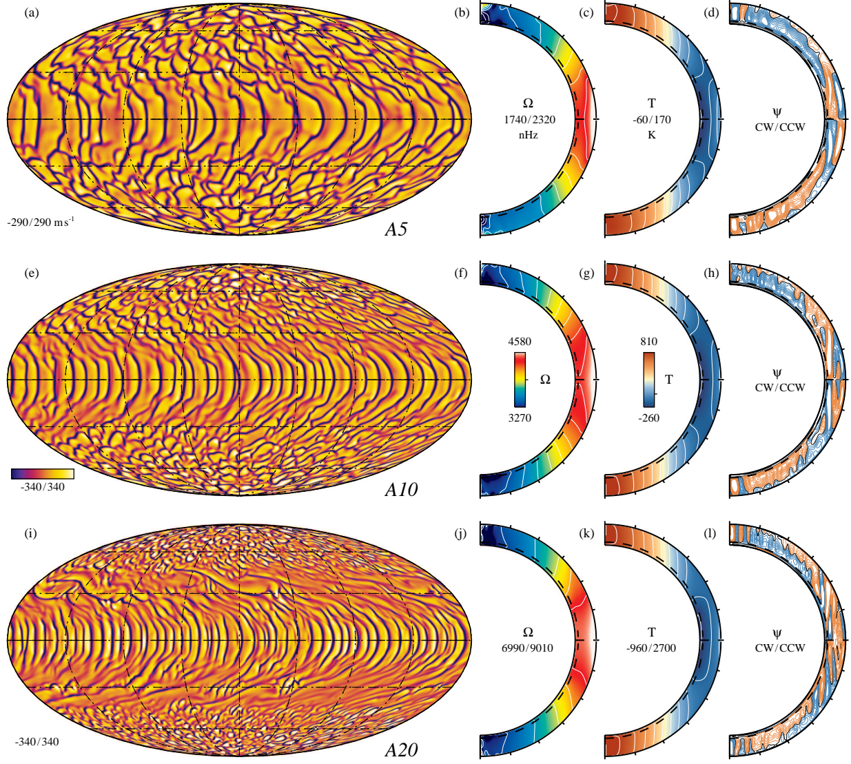
Figure 6.3: Overview of convective patterns, mean flows, and mean temperature fluctuations in selected Cases A. The first column of figures (a, e, i) display convective patterns in radial velocities near the upper boundary in turn for Case A5, Case A10, and Case A20. (b, f, j) the second column presents the time- and azimuthally-averaged angular velocity with radius and latitude, with the fast prograde equator in red and slower poles in blue. (c, g, k) azimuthally- and time-averaged temperature fluctuations (where the \ell = 0 component has been removed) with the warm poles in red tones and the cool equator in blue tones. (d, h, l) the streamfunction of the meridional flow ( \psi ), clockwise (CW) flows in red and counter-clockwise (CCW) flows in blue. The dashed line in the second, third and fourth columns delineates the beginning of the stable region.
