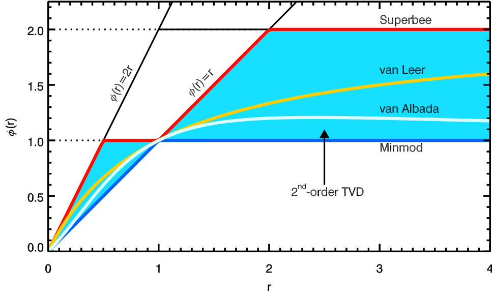
Figure 4.1: The space of second order total variation diminishing schemes is shaded in light blue, being bounded above by the superbee limiter (red) and from below by the minmod limiter (dark blue). The van Leer limiter is plotted in orange, and the van Albada limiter in gray. The abscissa r is the value of the ratio of adjacent derivatives and the ordinate \phi is the value of the limiter.
