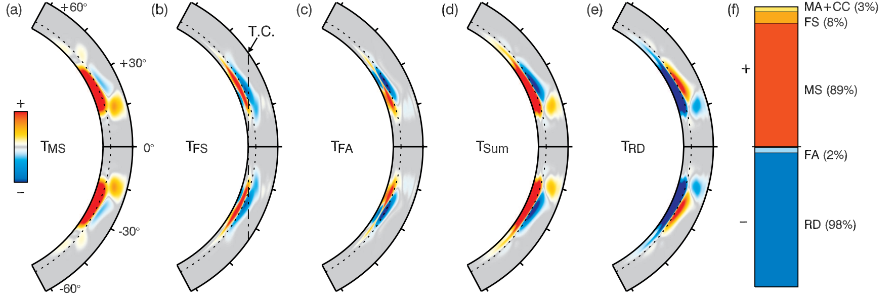
Figure 8.6: Generation of mean toroidal magnetic energy ( T_{ME} ) in Case A10m. The view is from \pm 60^\circ to emphasize the equatorial regions. Here only the dominant production terms are shown, namely (a) mean shear ( T_{MS} ), (b) fluctuating shear ( T_{FS} ), a cylinder tangent to the bottom of the domain (T. C.) is indicated (dashed line), (c) fluctuating advection ( T_{FA} ), (d) the sum T_{MS} + T_{FS} + T_{MA} + T_{FA} + T_{CC} , which largely act in concert to balance (e) the resistive diffusion of field ( T_{RD} ). All panels have identical scaling. The mean generation terms shown here contribute to the T_{ME} when positive (red), and destroy it if they are negative (blue). (f) The relative contribution of each term, with terms in red adding to the volume- and time-averaged toroidal energy generation and those in blue dissipating energy.
