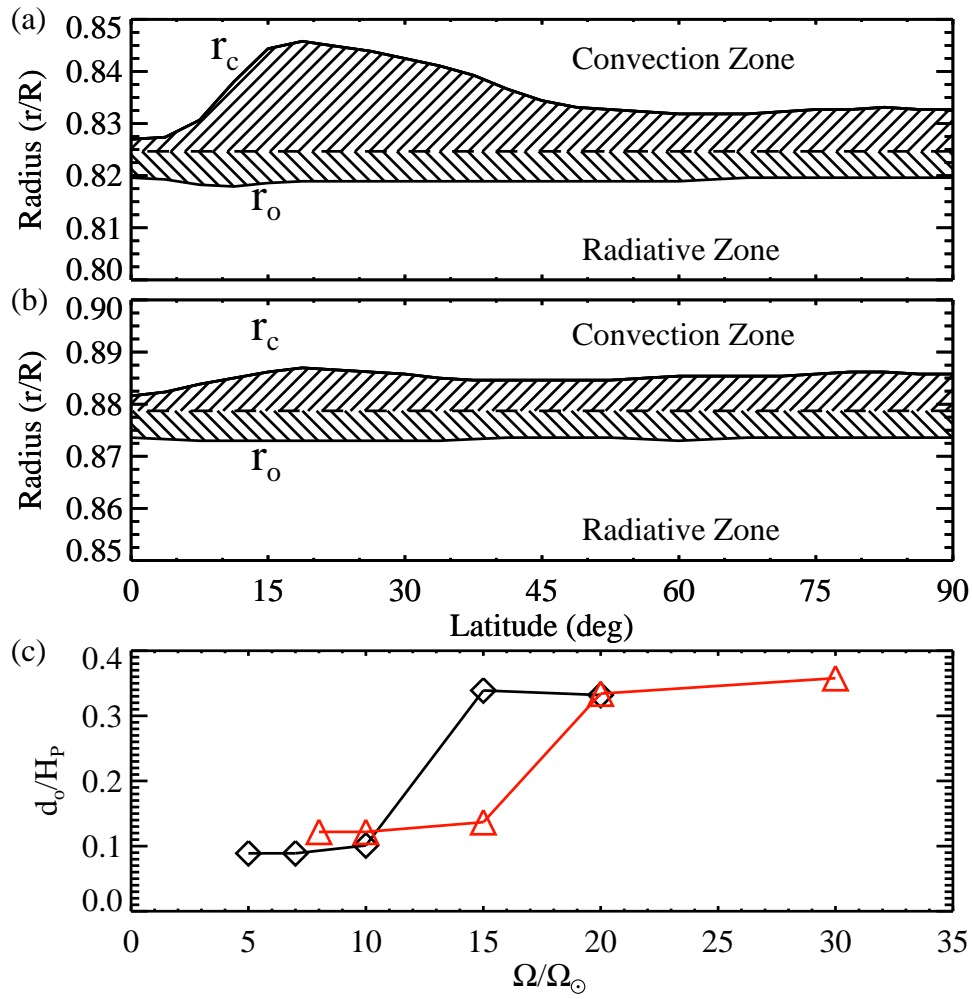
Figure 7.3: Changes in the radial extent of overshooting motions with latitude. Shown as a shaded region below r_{bcz} for case (a) Case A10 and (b) Case B10 . The radii where the enthalpy flux is negative encompasses the full shaded region. The radius at which there is a transition to the convection zone is denoted by r_c . The lower boundary of the overshooting motions is denoted by r_o . The scaling with rotation rate of the depth of the overshooting region relative to the pressure scale height at r_{bcz} ( d_o/H_p ) for cases A and B.
