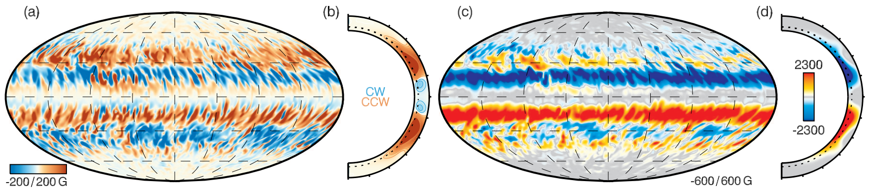
Figure 8.5: Snapshot of the magnetic field in Case A10m , coincident with radial velocities in Figure 8.3(e). (a) Radial component of the magnetic field ( B_r ) shown near the upper boundary, where multiple zonal bands are visible in the convection zone, (b) Mean poloidal field lines shown with radius and latitude, exhibiting the quadrupolar nature of the poloidal field. (c) Toroidal magnetic field ( B_\phi ) in the convection zone displaying the primary wreaths occupying lower latitudes and the secondary bands of field at higher latitudes. (d) Time- and azimuthally-averaged \langle B_\phi \rangle . The toroidal fields obtain their greatest amplitudes in the stable zone, where the peak strength of \langle B_\phi \rangle is 11 kG. Also evident is the radial dependence of the latitudinal connectivity of B_\phi , where the wreaths are connected in the stable zone but are disrupted in the convection zone by the presence of weak field of the opposite sense at mid-latitudes, as in (c).
