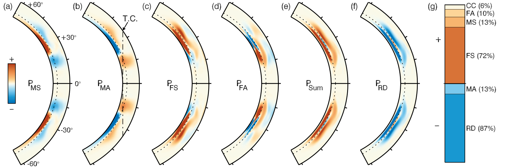
Figure 8.7: Generation of mean poloidal magnetic energy ( P_{ME} ) in Case A10m. The dominant production terms are shown, namely (a) mean shear ( P_{MS} ), (b) mean advection ( P_{MA} ), a cylinder tangent to the bottom of the domain (T. C.) is indicated (dashed line), (c) fluctuating shear ( P_{FS} ), (d) fluctuating advection ( P_{FA} ) and (e) the sum P_{MS} + P_{FS} + P_{MA} + P_{FA} + P_{CC} , with (f) the resistive diffusion of field ( P_{RD} ). The mean generation terms shown contribute to the P_{ME} when positive (red), and destroy it if negative (blue). (g) The relative contribution of each term, with those in red adding to the volume- and time-averaged poloidal energy generation and those in blue dissipating energy.
