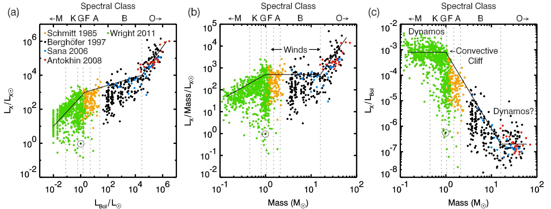
Figure 2.13: X-ray luminosity observations are displayed, showing such observations over the mass range of the main-sequence. (a) Average X-ray luminosity, L_X versus bolometric luminosity L_{Bol} , both normalized by their respective solar values. Spectral type is indicated along the top abscissa and demarked with thin dotted lines. The black line is meant to illustrate the mean slope of the three distinct ranges of behavior. The sources for the data are indicated in (a). (b) L_X to mass ratio plotted versus mass. This serves to highlight the region where L_X depends linearly on mass and is likely wind driven. (c) The ratio L_X/L_{Bol} versus mass, highlighting the mass range where L_X is linearly related to the L_{Bol} . The location of the Sun is plotted with its symbol \odot , showing its relatively low X-ray luminosity.
