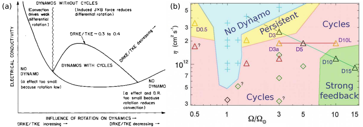
Figure 3.11: (a) A sketch of possible dynamo regimes with rotation rate and electrical conductivity, illustrating the cycling and persistent dynamo regimes as well as those without sustained dynamo action [adapted from Gilman (1983)]. (b) A set of numerical dynamo experiments carried out with varying Prandtl numbers and rotation rates, exhibiting many of the behaviors predicted in Gilman (1983) and some that were not, particularly at low rotation rate [adapted from Brown et al. (2011a)].
