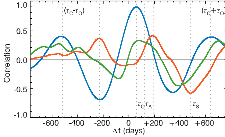
Figure 9.7: Temporal cross-correlations of volume-averaged magnetic energy generation rates for Case A20m . Cross-correlation of T_{MS} and P_{FS} in the stable zone (red) and convection zone (blue). Cross-correlation of T_{MS} between the stable and convection zones (green). Relevant time scales are indicated as average magnetic energy cycle time \tau_C , convective overturning time over the entire convection zone \tau_O , radial Alfvén wave \tau_A crossing time across the shell, and the polar-slip time \tau_S .
