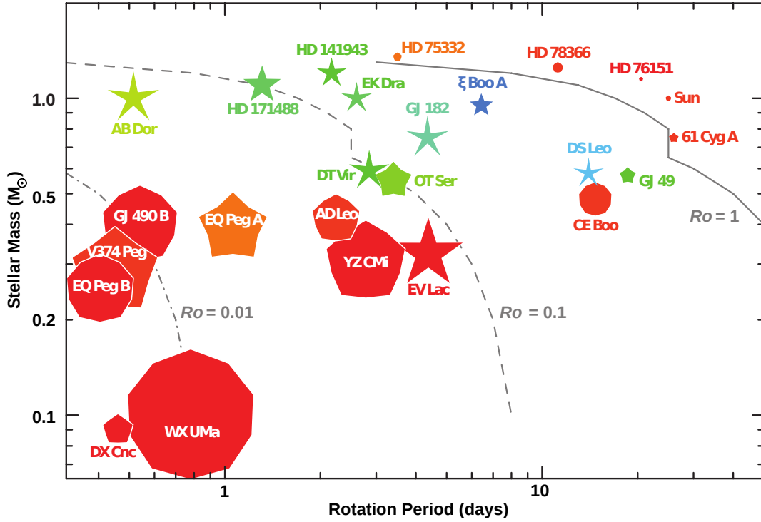
Figure 2.9: Global-scale morphology of spectropolarimetrically reconstructed magnetic fields on low-mass stars, as a function of stellar mass and rotation rate. Symbol size indicates rms magnetic field strength and symbol color illustrates field configurations, with blue for purely toroidal fields and red for purely poloidal fields. The symbol geometry is meant to depict the degree of axisymmetry of the poloidal field component, where the fully convex decagon indicates purely axisymmetric fields and the most concave star represents purely non-axisymmetric poloidal fields. The curves trace contours of constant Rossby number ( Ro = P/\tau_c ), with solid at Ro = 1 , dashed at Ro = 0.1 , and dash-dot at Ro = 0.01 (using convective turnover times \tau_c from Kiraga & Stepien (2007)). The smallest and largest symbols correspond to mean large-scale field strengths of 3 G and 1.5 kG on a logarithmic scale. (Adapted from Donati & Landstreet (2009)).
