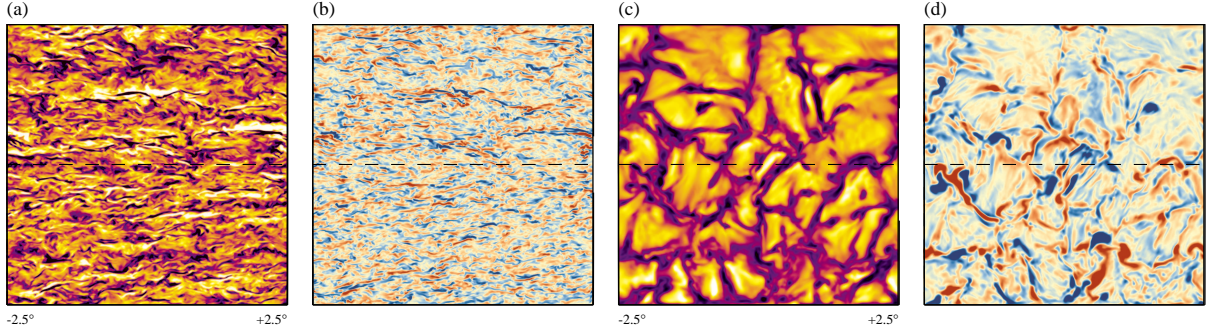
Figure 11.1: MHD simulations with CSS. Simulations of the magneto-rotational instability in spherical coordinates with (a) radial velocities and (b) radial magnetic field near the upper boundary of the simulation. An MHD convection simulation with (c) radial velocities and (d) radial magnetic field near its upper boundary.
