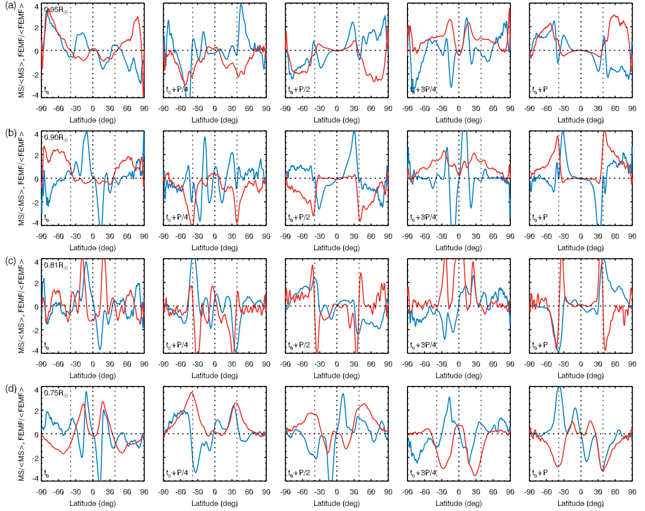
Figure 5.12: A comparison of the latitudinal regions of generation by the two primary toroidal and poloidal field production mechanisms at intervals of a quarter of the polarity cycle period in the average cycle. This serves to show the relative displacement of the two mechanisms, which may assist the wreaths in their equatorward propagation. The production of toroidal field is shown in blue, and the fluctuating azimuthal EMF is in red. The time series begins at t_0 and increments by a quarter of the polarity cycle period as one proceeds to the right. This is repeated for four depths: (a) 0.95 R_\odot , (b) 0.90 R_\odot , (c) 0.81 R_\odot , (d) 0.75 R_\odot .
