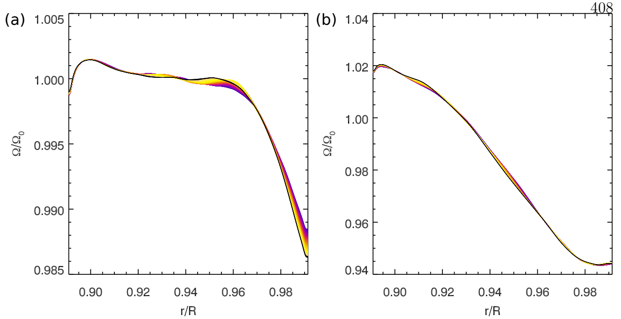
Figure 11.14: Shell-averaged angular velocity profiles with shear layers realized in CSS simulations. (a) A Sun-like star rotating at 10 \Omega_\odot , the color denotes the time evolution of the angular velocity with several hundred days represented, showing the presence of a near surface shear layer. (b) A Sun-like star rotating at 3 \Omega_\odot , lacking a shear layer due to the larger Rossby number throughout the domain.
