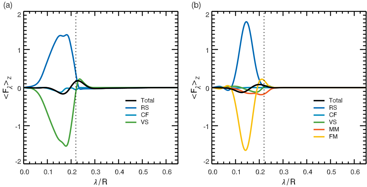
Figure 10.6: A comparison of angular momentum transport mechanisms in Cases H4 and M4 . The cylindrically-averaged angular momentum fluxes \langle F_\lambda \rangle_z are shown with proportional cylindrical radius \lambda/R for (a) Case H4 and (b) Case M4 , in units of 10^{40} \text{ g s}^{-2} . The flux components are the total flux (black), the Reynolds stress (RS; blue), the advection by the meridional circulation (MC; teal), viscous stresses (VS; green), mean Maxwell stresses (MM; red), and fluctuating Maxwell stresses (FM; orange).
