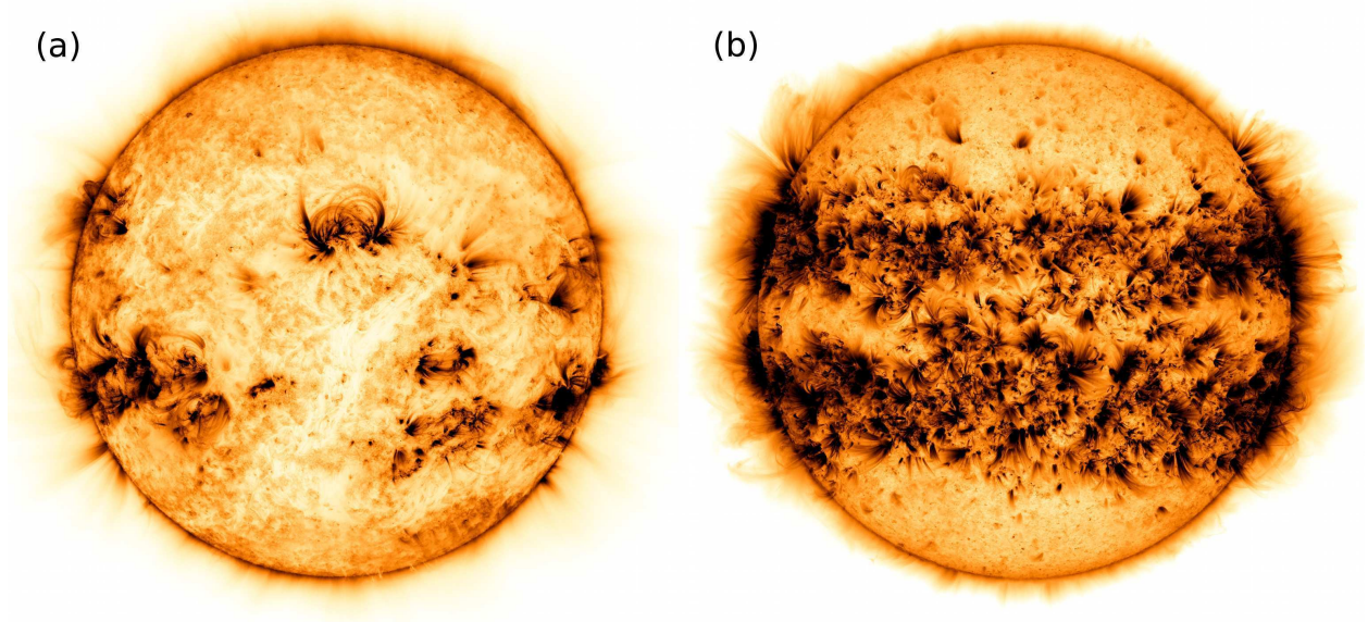
Figure 1.3: (a) The solar transition region imaged in the 171 Å channel with AIA on SDO from 20 July 2013, dark tones indicate areas of high emission and light tones low emission. (b) A composite of 25 images from the period between 16 March 2012 to 15 March 2013 in the same Fe IX resonance line, illustrating latitudinal bands of magnetic activity (NASA/SDO/AIA & S. Wiessinger).
