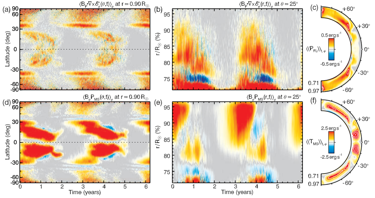
Figure 5.9: A comparison of the temporal evolution of the poloidal magnetic energy production through the fluctuating EMF as P = \mathbf{B}_P \cdot \nabla \times \mathcal{E}'_\phi and toroidal magnetic energy production by mean shear with T = B_\phi P_{MS} in D3S. All cycles have been stretched to the the same time span and then averaged to allow the progression of an average cycle to be ascertained. (a) Poloidal magnetic energy generation P in the upper convection zone shown with latitude and time in cylindrical projection, illustrating the strong field generation above about \pm 30^\circ and the weak generation that accompanies the equatorward propagation of the large toroidal wreaths. (b) P plotted with depth r/R_\odot at a latitude of 25^\circ . The tapering with depth arises from the strong radial dependence of \mathbf{B}_P , with a downward direction of propagation. (c) P averaged over the entire cycle rendered in the meridional plane. (d) Toroidal magnetic energy generation T exhibited over the average cycle and with latitude in cylindrical projection, showing the equatorward migration of field generation. (e) T in depth and time at a latitude of 25^\circ , with two zones of migration evident. (f) T averaged over the entire cycle, where the equatorial and polar regions represent spatially separated zones of generation.
