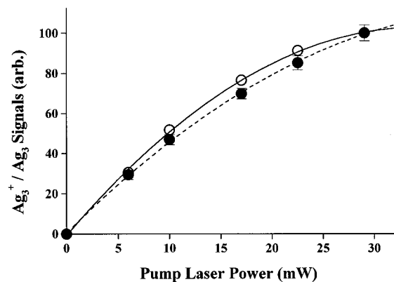
Figure 5. Pump power dependence of the Ag 3 + yield (—○—) with the probe laser off, and the Ag 3 + ion yield (---●---) at Δt = 1 ps and with a fixed probe intensity, obtained with a 410-nm pump and 410-nm probe.
