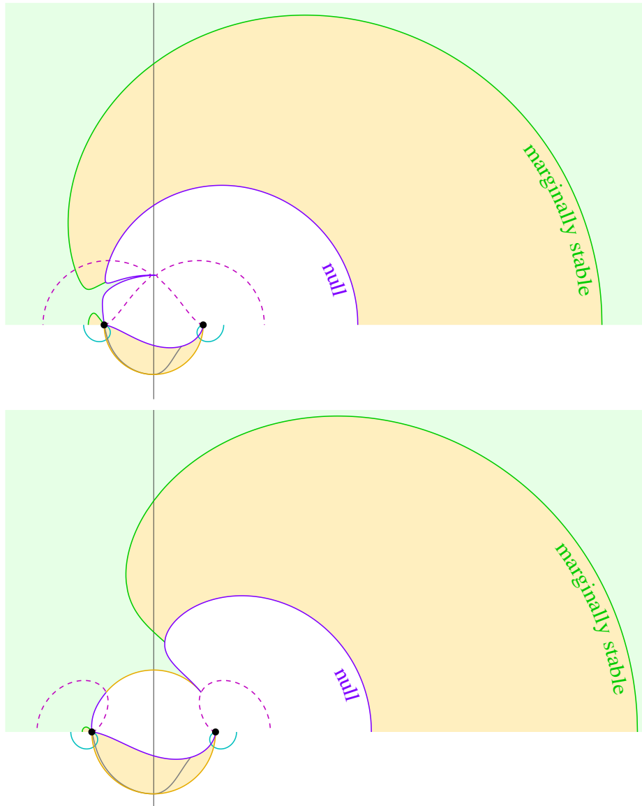
Figure 23.5 As Figure 23.4, but for a Kerr black hole with spin (top) slightly super-extremal ( a = 1.001M ), and (bottom) super-extremal ( a = 1.25M ). Ergospheres, sisy tubes, and singularities are shown as in Figure 9.4.
