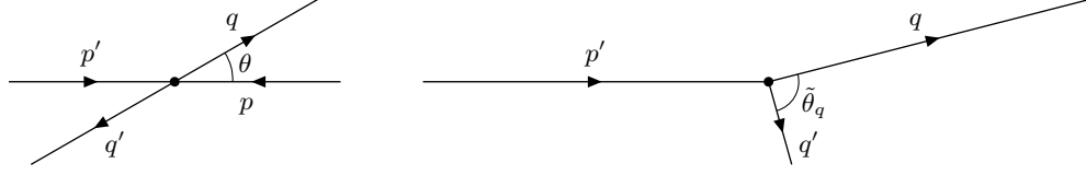
Figure 47.11 Annihilation of a spinor-antispinor pair into another spinor-antispinor pair (left) in the centre-of-mass frame, and (right) in the rest frame of the incoming p spinor. This figure is similar to Figure 47.9 but with q \rightarrow p' \rightarrow q' \rightarrow q . The lengths and directions of the lines are proportional to the spatial momenta. In the centre-of-mass frame, the outgoing q\bar{q} pair are deflected by angle \theta from the incoming p\bar{p} pair. In the rest frame of the incoming p spinor, the angle between the outgoing q\bar{q} pair is \tilde{\theta}_q , equation (47.114). If the p and q spinors are identical, then the situation p + \bar{p} \rightarrow p + \bar{p} where a spinor-antispinor pair annihilate into another pair is indistinguishable from Coulomb scattering of a spinor and antispinor.
