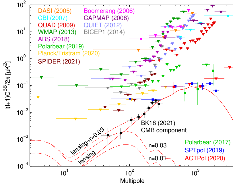
Figure 38.1 CMB B -mode polarization upper limits and detections (BICEP/Keck Collaboration, 2021, Fig. 7). Lines show theoretical predictions for the lensing B -modes (solid red) which peak at arcminute scales \ell \sim 1000 , and for primordial gravitational wave B -modes (dashed red) for two values of the tensor-to-scalar ratio r , peaking at degree scales \ell \sim 80 .
