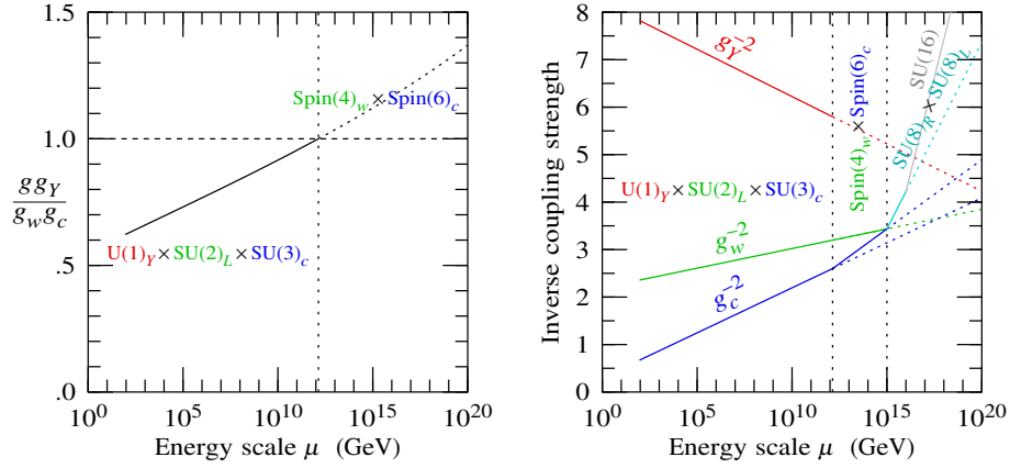
Figure 50.2 (Left) Symmetry breaking of the Pati-Salam group \text{Spin}(4)_w \times \text{Spin}(6)_c to the standard model should occur where gg_Y/(g_w g_c) = 1 , which happens at energy scale \mu = 10^{12} GeV, equation (50.70). (Right) Running of the standard-model coupling parameters g_Y , g_w , and g_c with renormalization energy scale \mu , equation (50.60). The solid blue line ( g_c^{-2} ) tracks the colour force \text{SU}(3)_c below the \text{Spin}(4)_w \times \text{Spin}(6)_c transition energy, then \text{Spin}(6)_c above the transition energy. The solid green line ( g_w^{-2} ) tracks the weak force \text{SU}(2)_L below the transition energy, then \text{Spin}(4)_w above the transition energy. The weak and colour couplings g_w and g_c merge at \mu \approx 10^{15} GeV. The solid cyan line tracks the gauge group \text{SU}(8)_R \times \text{SU}(8)_L above the weak-colour merger scale \mu \approx 10^{15} GeV, equation (50.70). Grand symmetry breaking from \text{SU}(16) , mediated by the grand Higgs field \mathbf{T} , equation (50.31), could occur at any energy at or above the merger scale \mu \approx 10^{15} GeV. The grey line tracks the grand unified group \text{SU}(16) with grand symmetry breaking taken at \mu = 10^{16} GeV. The lines are straight lines when g^{-2} is plotted versus log energy.
