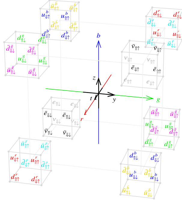
Figure 49.1 A generation (the electron generation) of 64 fermions arranged according to their \text{Spin}(11,1) tyzrgb charges. This is similar to Figure 48.1, but with the addition of the t -bit, with t -bit-up directed out of the page. Whereas in the \text{Spin}(10) Figure 48.1 each fermion was a 2-component Weyl fermion, here the Weyl components are distinguished by their Dirac boost ( \uparrow or \downarrow ) and spin ( \uparrow or \downarrow ) bits. A right-handed Weyl fermion has Dirac bits \uparrow\uparrow or \downarrow\downarrow , while a left-handed Weyl fermion has Dirac bits \downarrow\uparrow or \uparrow\downarrow . Flipping the t -bit of a fermion flips the fermion to its antifermionic partner of opposite boost and the same spin. Flipping all 6 tyzrgb bits of a fermion flips its Dirac boost and spin bits, thereby transforming the fermion to its Weyl companion.
