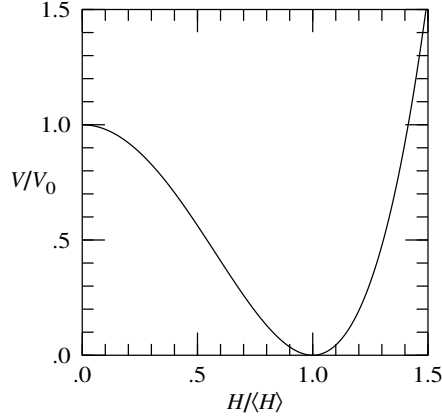
Figure 50.1 Mexican hat quartic potential V of a Higgs field of magnitude H .
