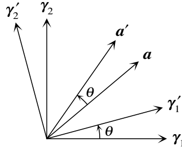
Figure 13.4 Right-handed rotation of a vector \mathbf{a} by angle \theta in the \gamma_1\gamma_2 -plane. A rotation in the geometric algebra is an active rotation, which rotates the axes \gamma_a \rightarrow \gamma'_a while leaving the components a^a of a multivector unchanged, equation (13.54). In other words, multivectors \mathbf{a} are considered to be attached to the frame, and a rotation bodily rotates the frame and everything attached to it.
