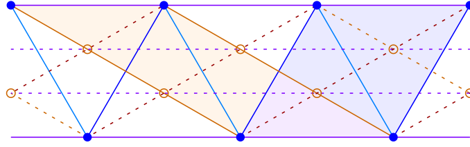
Figure 39.2 Standard (blue) and self-dual m = 1 (orange) SU(3) lattices. Vertices with integral coordinates are coloured blue; those with nonintegral fraction coordinates are coloured orange. The blue-shaded region (two equilateral triangles) is a fundamental tile of the standard SU(3) lattice, generated by the two simple roots \alpha_1 and \alpha_2 , signified by the purple and blue solid lines. Altogether there are \frac{1}{2}n(n+1) = 3 simple roots of length squared equal to two, signified by the purple/blue/cyan solid lines, which represent massless gauge bosons; the simple roots are raising operators in one direction, lowering operators in the opposite direction, for a total of n(n+1) = 6 degrees of freedom. The self-dual (orange) lattice contains spinor roots (dashed orange/maroon lines) of length squared (km-1)/k = 2/3 , equation (39.74), which is less than two, which would represent tachyonic (negative mass-squared) gauge bosons if they were present. These tachyonic roots are eliminated by taking the (km = 3) -fold cover of the self-dual lattice. The orange-shaded region is a fundamental tile of the 3-fold cover of the self-dual lattice, generated by the spinor root km\sigma_p = 3\sigma_2 together with the simple root \alpha_2 , signified by the orange and purple solid lines. The 3-fold cover of the self-dual lattice is again self-dual, and its nearest-neighbour roots of length squared two coincide with those of the standard lattice.
