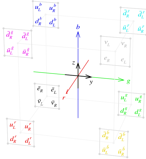
Figure 48.1 A generation (the electron generation) of 32 fermions arranged according to their Spin(10) yrgb charges. The eight squares are distinguished by their colour rgb bits, with r -bit-up directed out of the page, g -bit-up directed rightward, and b -bit-up directed upward. The fermions in each of the eight squares are distinguished by their weak yz bits, with y -bit-up directed rightward, and z -bit-up directed upward. A Spin(11, 1) version of this figure is Figure 49.1.
