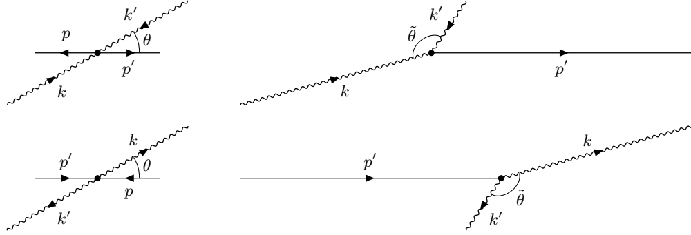
Figure 47.7 Spinor-antispinor (top) creation, and (bottom) annihilation, (left) in the centre-of-mass frame, where p_a + p'_a = k_a + k'_a = 0 , and (right) in the rest frame of the spinor, where p_a = 0 . In the centre-of-mass frame, the angle between the incoming and outgoing pairs is \theta . In the rest frame of the incoming p spinor, the photon is deflected by angle \tilde{\theta} , equation (47.59). The lengths and directions of the lines are proportional to the spatial momenta. The parameters of the collision in this instance are \eta = \text{atanh } \frac{3}{5} and \theta = \frac{\pi}{6} .
