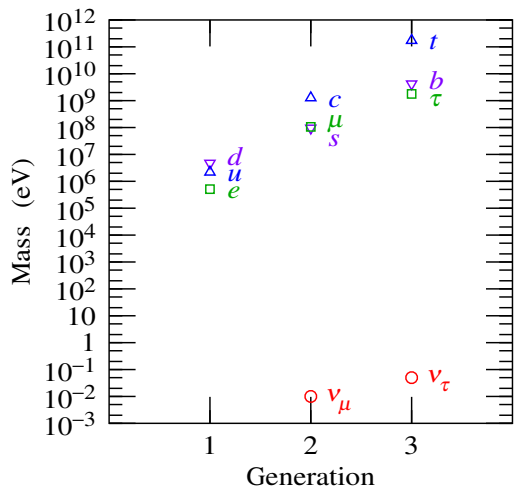
Figure 48.2 Masses of fundamental fermions, Table 48.2. Neutrino masses, and their assignment to generation, remain uncertain.
