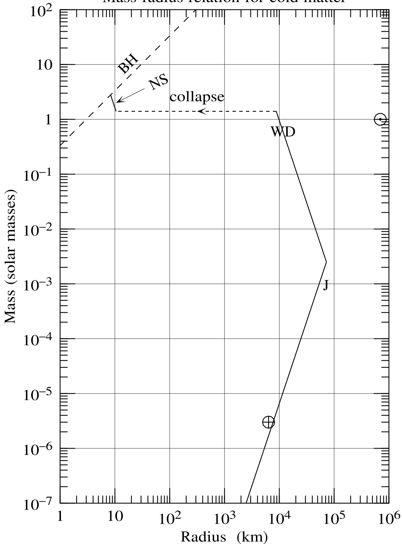
Mass-radius relation for cold matter
