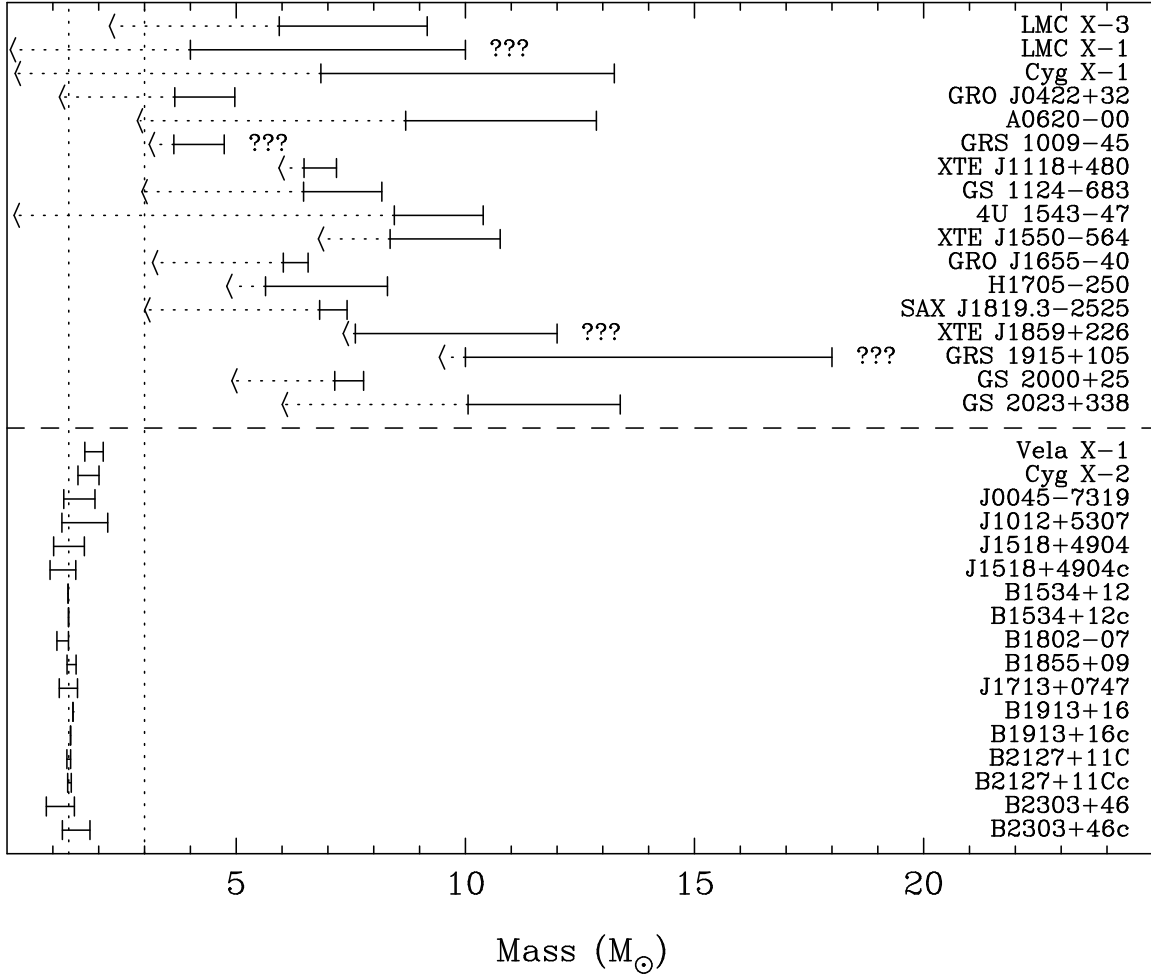
Figure 1: Summary of black hole masses, and selected neutron star masses. The arrowed dotted lines indicate mass functions (product of the mass and the sine of the inclination angle of the orbital plane).
