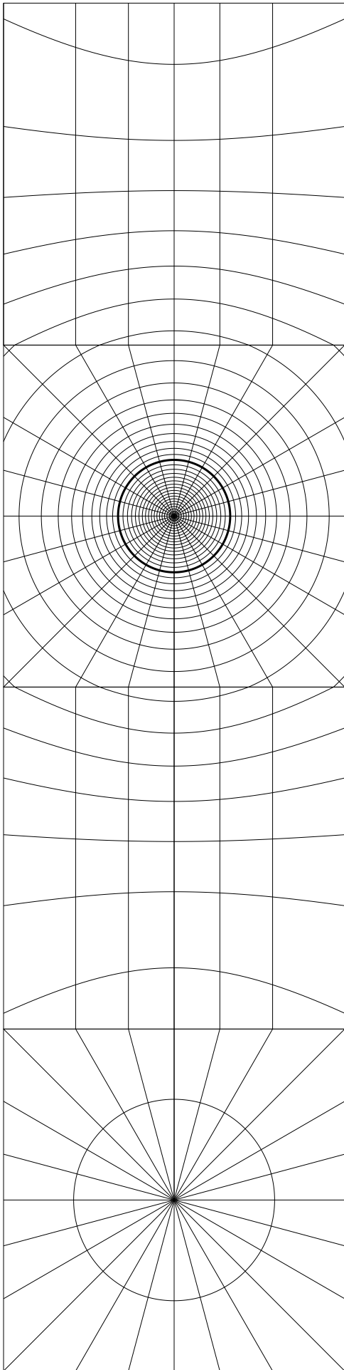
Relativistic ( v/c = 0.95 )
