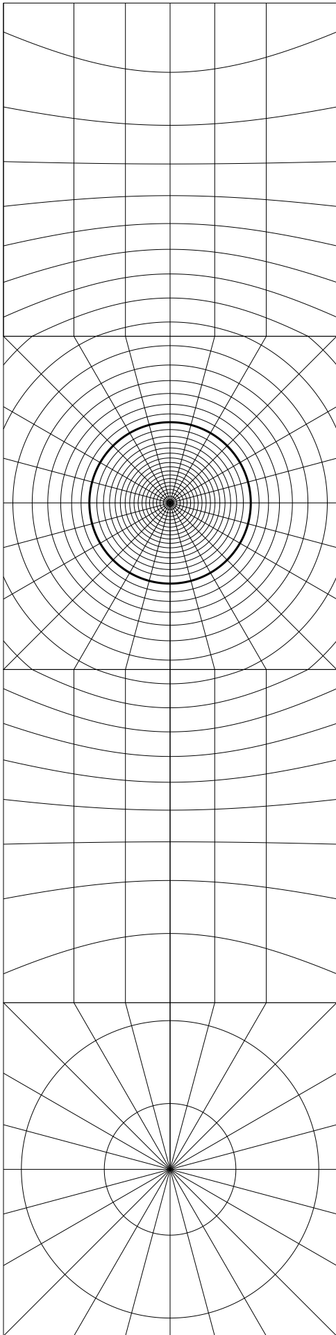
Relativistic ( v/c = 0.9 )
