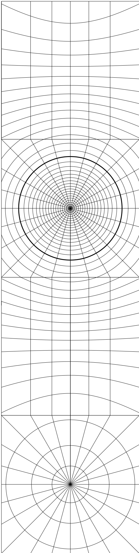
Relativistic ( v/c = 0.8 )
