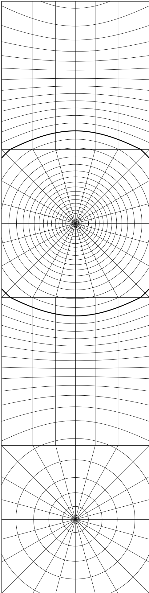
Relativistic ( v/c = 0.6 )
