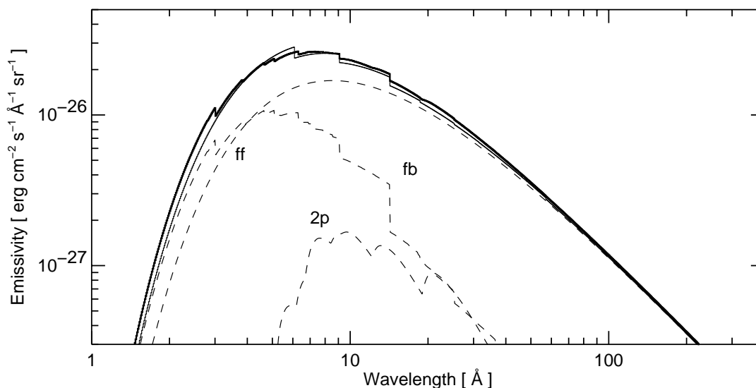
FIG. 6.—Comparison of the continuum emissivity predicted by CHIANTI (thick line) at a temperature of 1 \times 10^7 K with that obtained through the analytic approximations of Mewe et al. (1986). The individual contributions of the CHIANTI free-free (ff), free-bound (fb), and two-photon (2p) continua are indicated with dashed lines.
