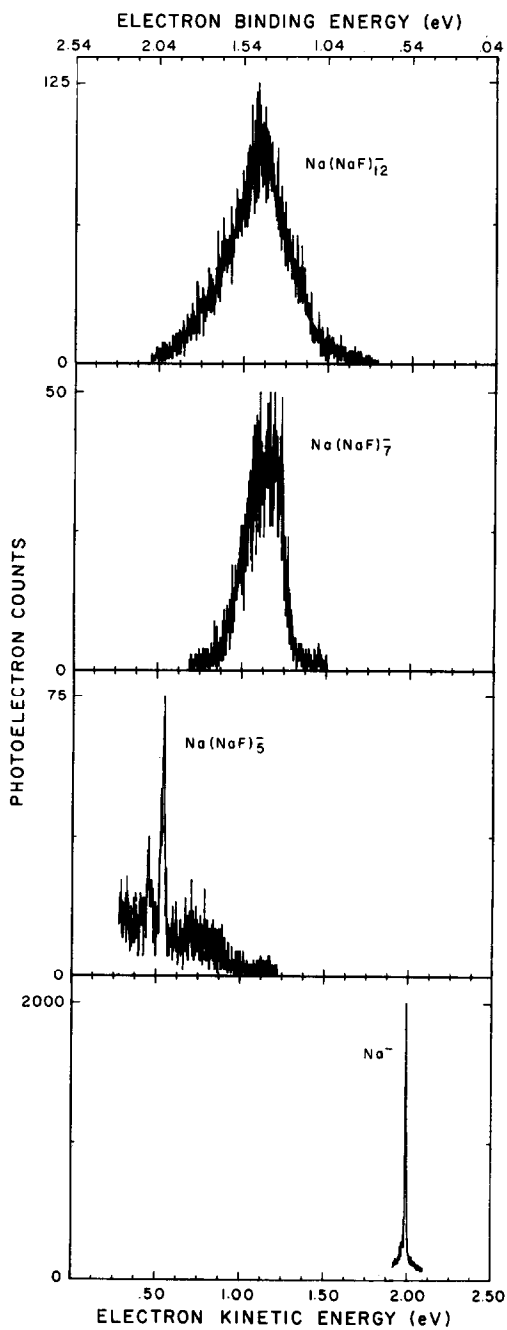
Fig. 3. Photoelectron spectra for \text{Na}(\text{NaF})_n^- ions at 488 nm.
