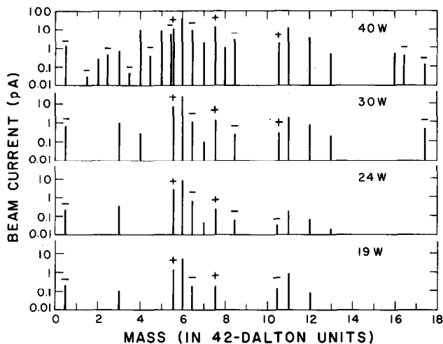
Fig. 1. Negative ion mass spectrum for \text{Na}_n\text{F}_n^- produced in a flowing afterglow ion source for different crucible heating power levels. The helium pressure was 0.6 torr and the ion flight path in the flow tube was 30 cm. The (\text{NaF})_n^- occur at integer multiples of 42 daltons. The \text{F}(\text{NaF})_n^- are marked with a minus sign (-) on this figure, and the \text{Na}(\text{NaF})_n^- are denoted by a plus sign (+). Clusters were observed up to about n = 17 , but the mass resolution does not permit precise identification of the ions above n = 13 .
