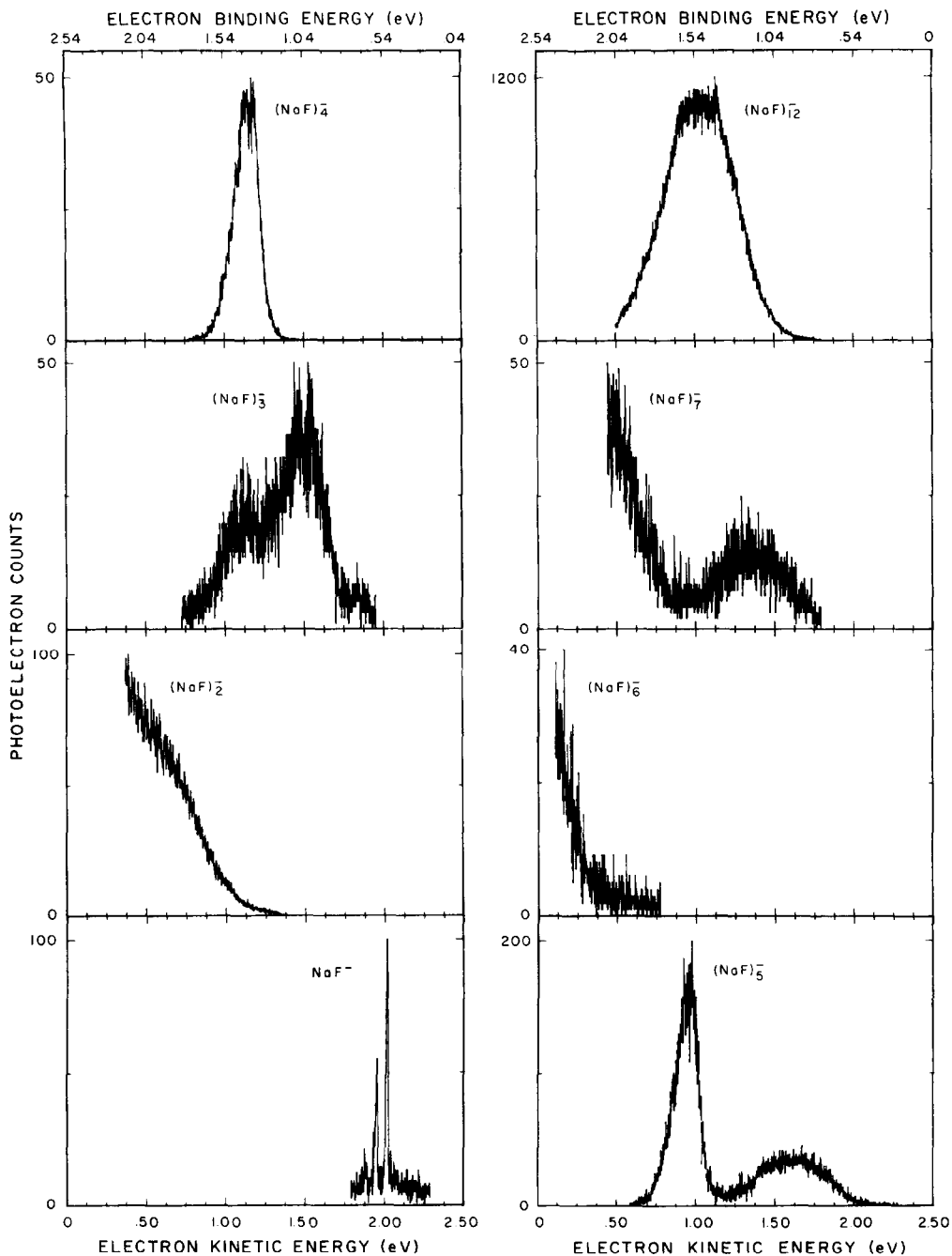
Fig. 2. Photoelectron spectra for (\text{NaF})_n^- ions at 488 nm. [The (\text{NaF})_6^- data were actually obtained at 454 nm because of the high electron binding energy in this case, and the electron energy scale was shifted by 0.070 eV to facilitate comparisons with the other spectra.]
