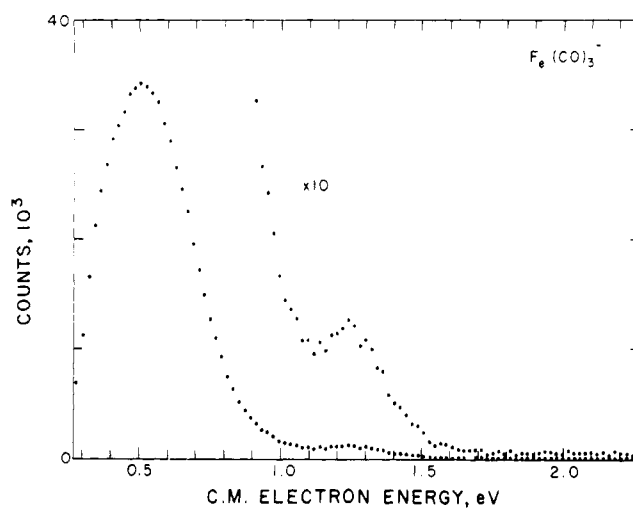
Figure 3. Photoelectron spectrum of \text{Fe(CO)}_3^- ions obtained with 2.54-eV photons. Spacing between data points is approximately 20 meV. The breadth of the feature indicates a substantial geometry change between anion and the neutral. The falloff in electron counts near 0.4 eV is largely instrumental.
