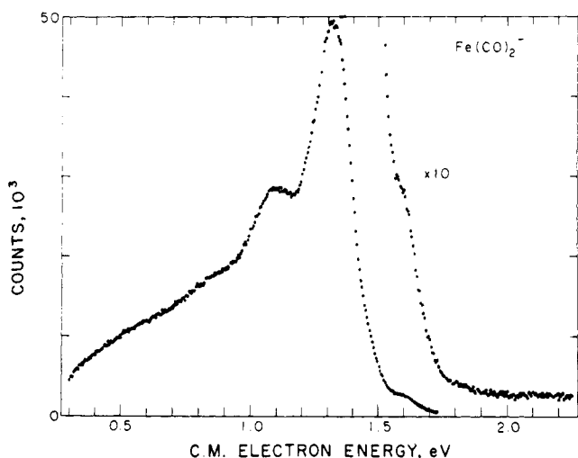
Figure 2. Photoelectron spectrum of \text{Fe(CO)}_2^- ions obtained with 2.54-eV photons. Spacing between data points is 5 meV. See text for details.
