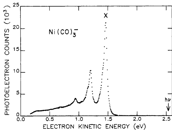
Figure 3. Photoelectron spectrum of \text{Ni}(\text{CO})_3^- obtained with 2.540 eV photons and an ion current of 6.0 nA; the electron affinity is again determined from the peak labeled X.
