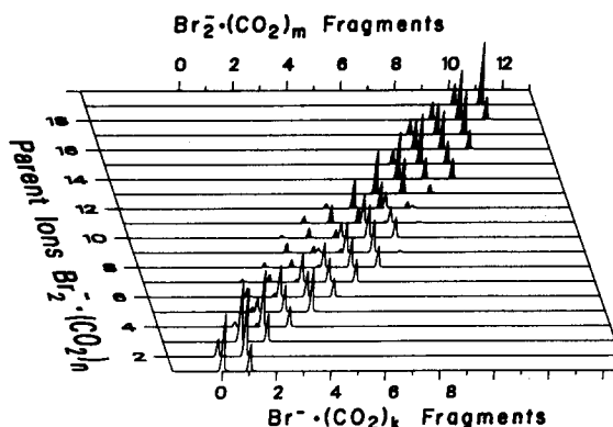
FIG. 5. A schematic representation of the ionic photofragments from \text{Br}_2^-(\text{CO}_2)_n , n = 1-19 , at 700 nm. The peaks lying along a given horizontal line represent the ionic photofragments from a given parent ion. \text{Br}^- based photofragments are unshaded and are labeled by the axis at the bottom. \text{Br}_2^- based photofragments are shaded and labeled by the axis at the top.
