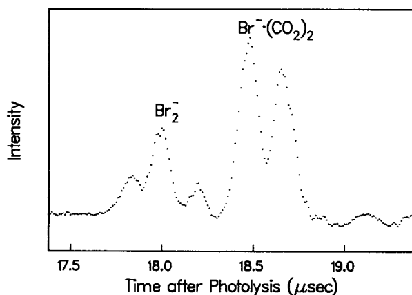
FIG. 4. Two ionic photofragments, \text{Br}_2^- (158, 160, and 162 amu for ^{79}\text{Br}_2^- , ^{79}\text{Br}^{81}\text{Br}^- , and ^{81}\text{Br}_2^- , respectively) and \text{Br}^-(\text{CO}_2)_2 (167 and 169 amu for the ^{79}\text{Br}^- and ^{81}\text{Br}^- isotopes, respectively), arising from the photofragmentation of \text{Br}_2^-(\text{CO}_2)_5 at 700 nm.
