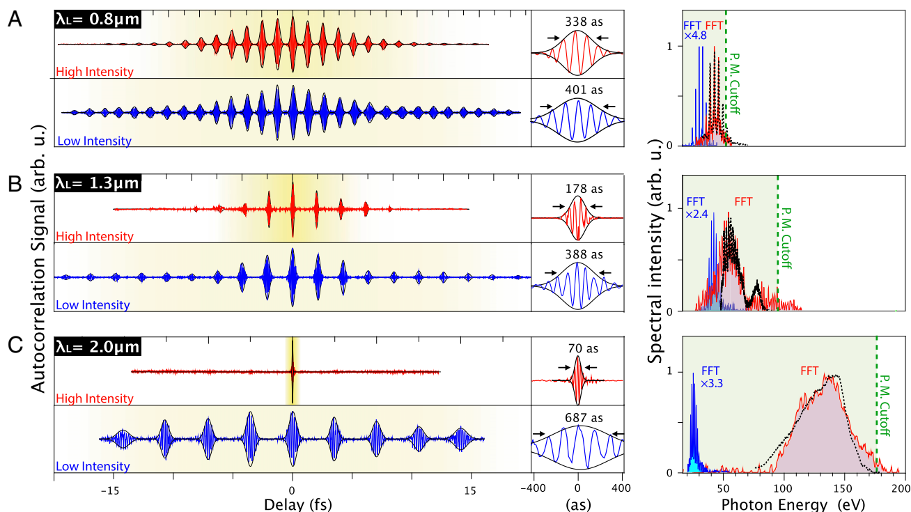
Fig. 2. Comparison of the experimental HHG autocorrelation data (normalized) from Ar driven by \sim 10 cycle laser pulses at wavelengths of (A) 0.8 \mu\text{m} , (B) 1.3 \mu\text{m} , and (C) 2 \mu\text{m} for high and low laser intensity conditions (red and blue lines). (Left) Field autocorrelation of the HHG field and enlarged view near time 0 with the coherence time of the central pulse envelope. The temporal phase-matching window is highlighted in yellow. Note that the bandwidth-limited pulse duration is half of this coherence time. (Right) HHG spectra obtained from the FFT of the field autocorrelation traces (filled-area plots), showing excellent agreement with the experimental spectra (black dotted lines). The low-intensity spectra are enhanced to see their fine structure. The predicted phase-matching cutoffs are also shown (green dashed lines).
