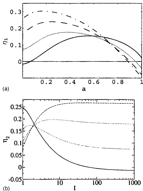
FIG. 4. Relative errors \eta_1 as a function of the scaled width a (panel a) and \eta_2 as a function of the scaled intensity I (panel b) for different input powers, P=3 (solid line), P=5 (dotted line), P=10 (dashed line), P=20 (dotted-dashed line).
