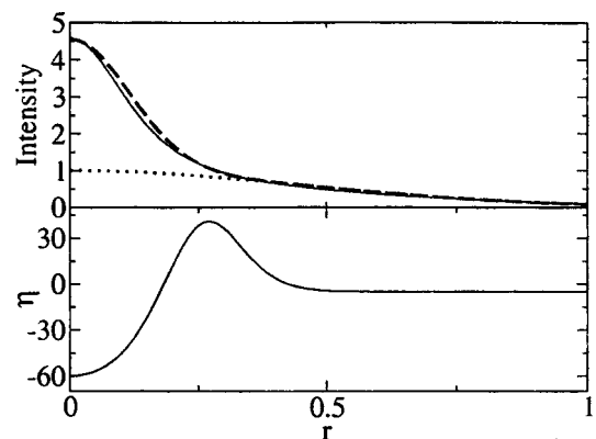
FIG. 6. The upper panel contains an example of the intensity distribution obtained from simulation (solid line) for P=5 and \xi = 0.2 . The distribution can be fitted by the superposition of two Gaussians (dashed line). One for the inner part, and the other for the background (dotted line). The lower panel contains the result of the operation in Eq. (44). Note that the region where the dashed line tends toward the dotted line (inner and outer part join), is where the maximum of the function \eta is located.
